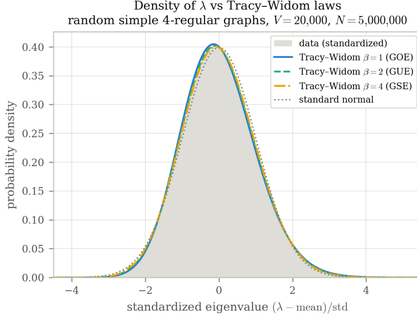
FIGURE 3.1. Standardized empirical density of the largest non-trivial eigenvalue over 5 \times 10^6 random simple 4-regular graphs on V = 20,000 vertices, against the standardized Tracy-Widom \beta = 1, 2, 4 densities and the standard normal.
