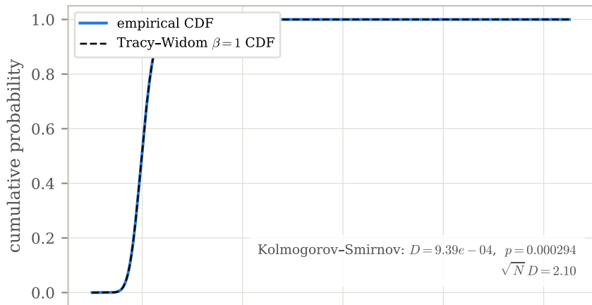
Empirical CDF vs Tracy-Widom \beta=1 random covers of K_5 - e , V=10,000 , N=5,000,000
