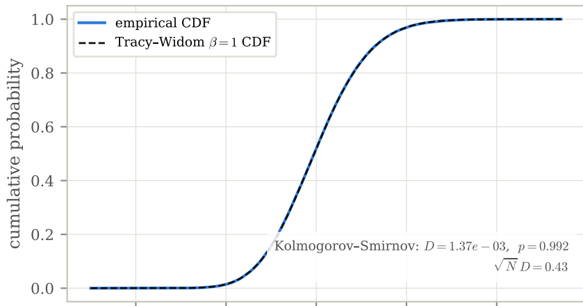
Empirical CDF vs Tracy-Widom \beta = 1 random simple 4-regular graphs, V = 500,000 , N = 100,000 (MATLAB)
