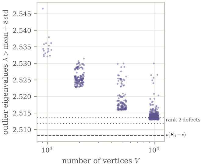
The defect band above \rho
