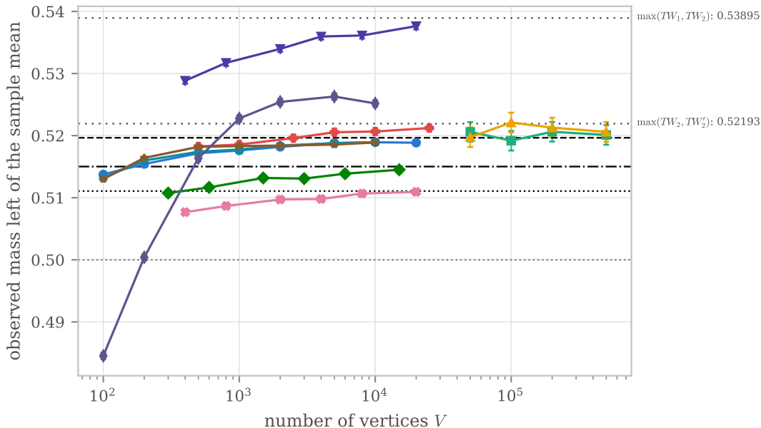
MNS's discriminating statistic: mass left of the mean (binomial error bars; smaller than markers at N \geq 1\text{M} )
