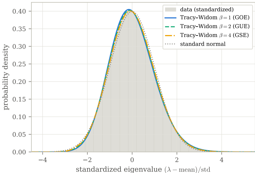
Density of \lambda vs Tracy-Widom laws random covers of K_5 , V = 10,000 , N = 5,000,000
