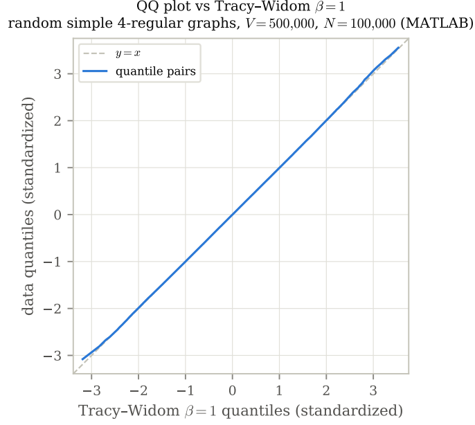
FIGURE 3.2. Quantile-quantile plot of 10^5 samples at V = 500,000 against \widetilde{TW}_1 , probability range 10^{-4} to 0.999.
