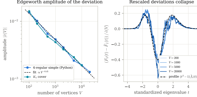
FIGURE 3.6. The approach to the limit. Left: the amplitude \hat{c}(V) of the deviation of the standardized empirical distribution from \widehat{TW}_1 , for the simple 4-regular and K_5 cover families, with the fitted power law. Right: the deviations at four sizes, rescaled by \hat{c}(V) , collapse onto the fixed profile (t^2 - 1)\tilde{f}_1(t) of a skewness deficit.
