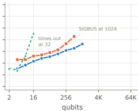
Grover
