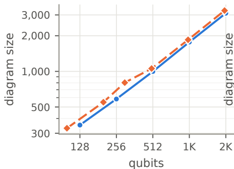
Grover
