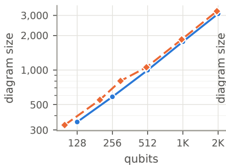
Grover
