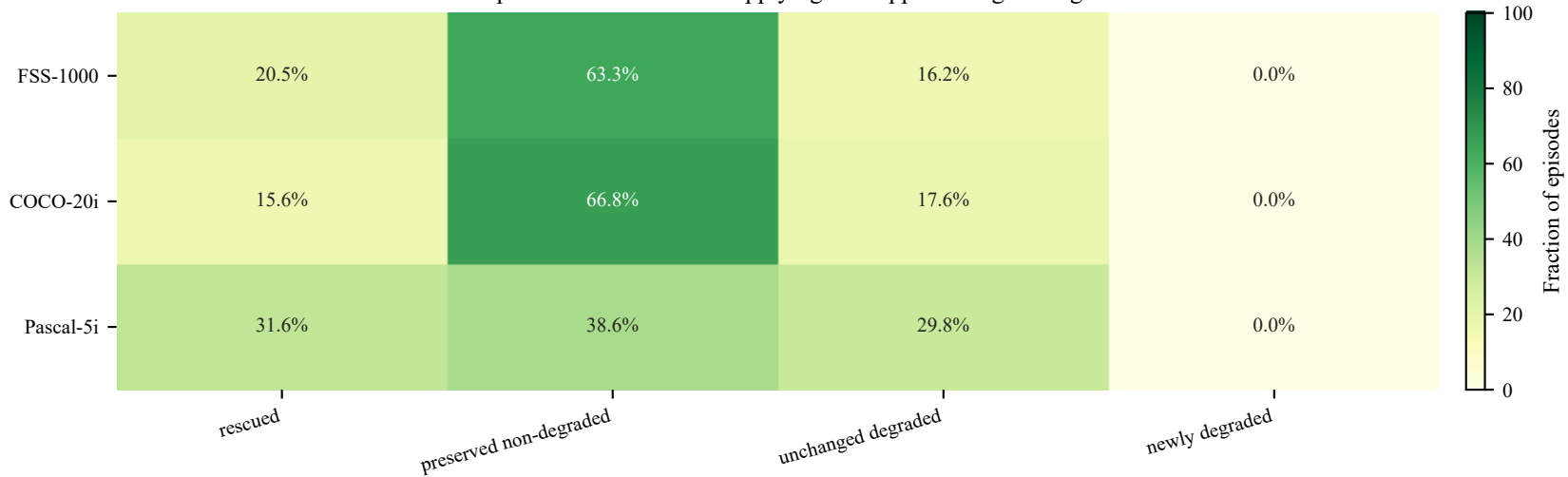
Per-episode transitions after applying the support-foreground gate
