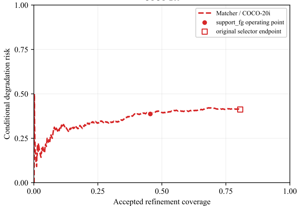
COCO-20i
