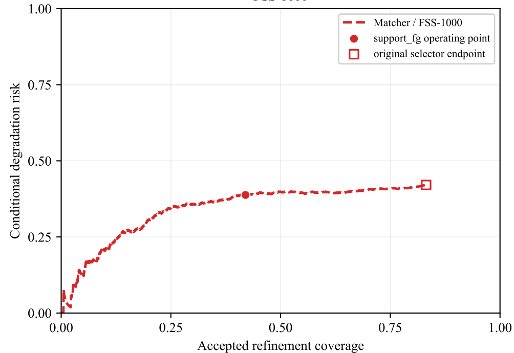
FSS-1000
