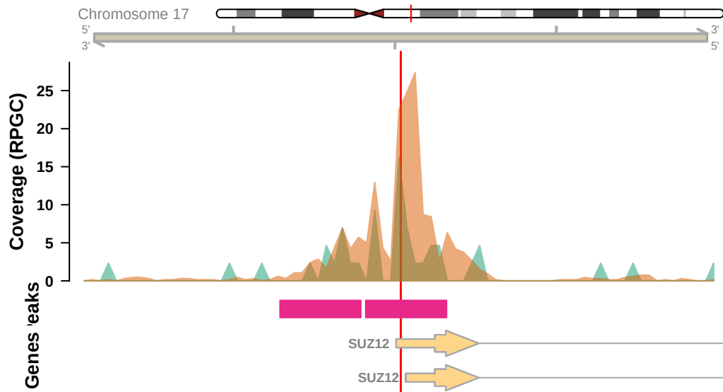
rs527723504 (SUZ12),Promoter (&lt;=1kb)
