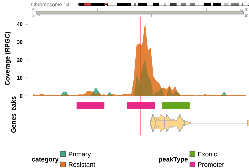
rs2741732 (METTL17),Promoter (<=1kb)
