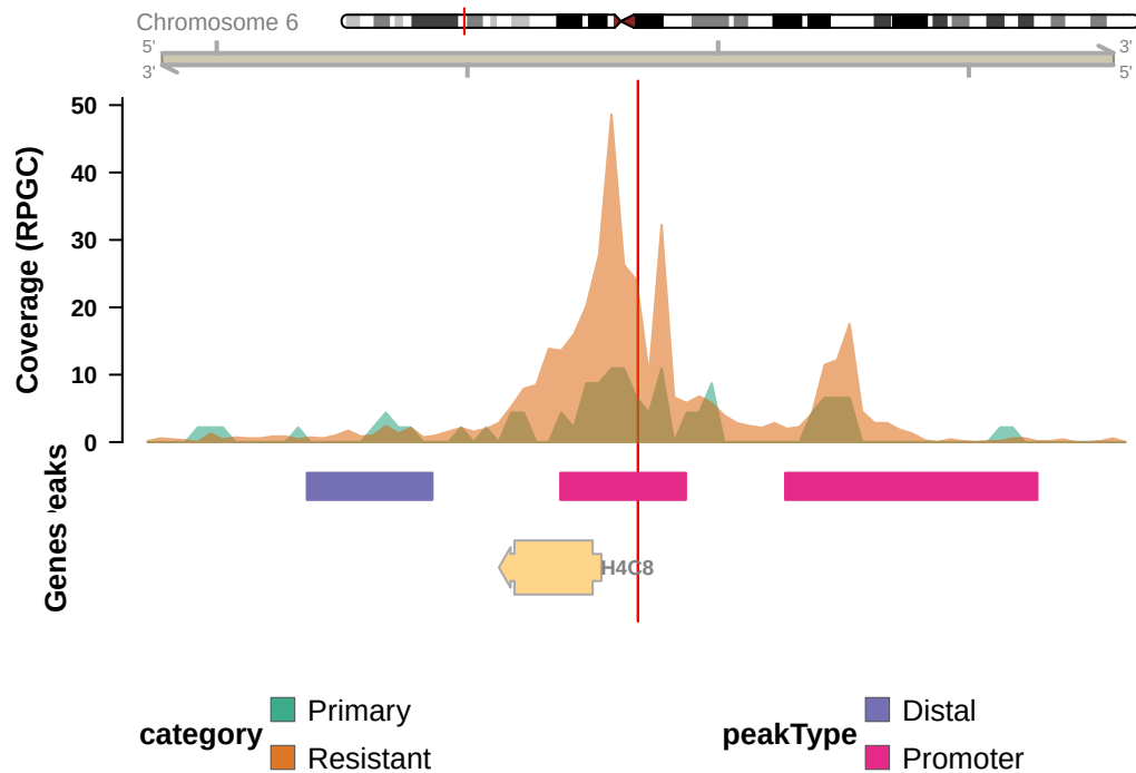
rs16891518 (H4C8),Promoter (&lt;=1kb)
