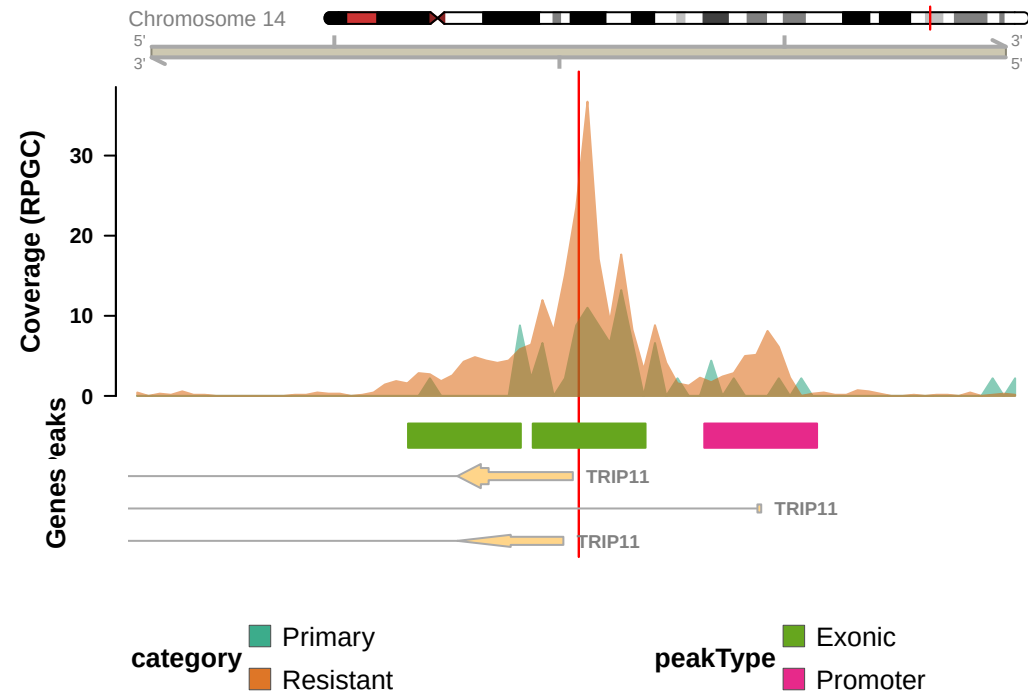
rs112899205 (TRIP11),Promoter (<=1kb)
