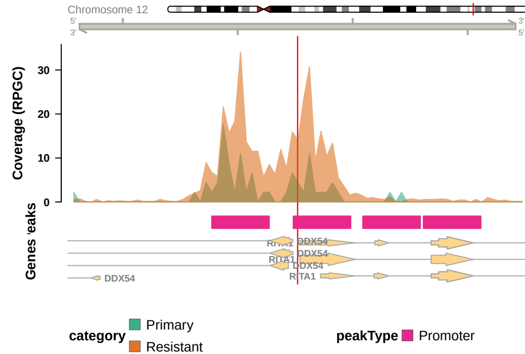
rs11066508 (RITA1),Promoter (<=1kb)
