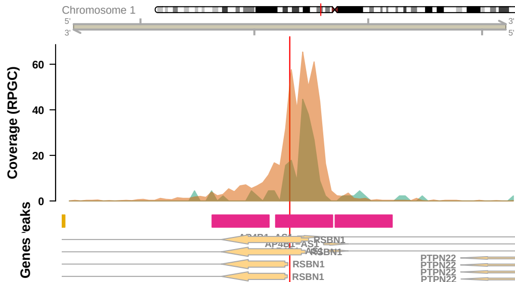
rs192007948 (RSBN1),Promoter (&lt;=1kb)
