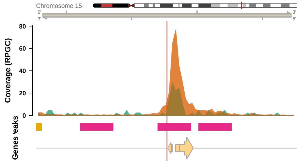
rs2301273 (STOML1),Promoter (&lt;=1kb)
