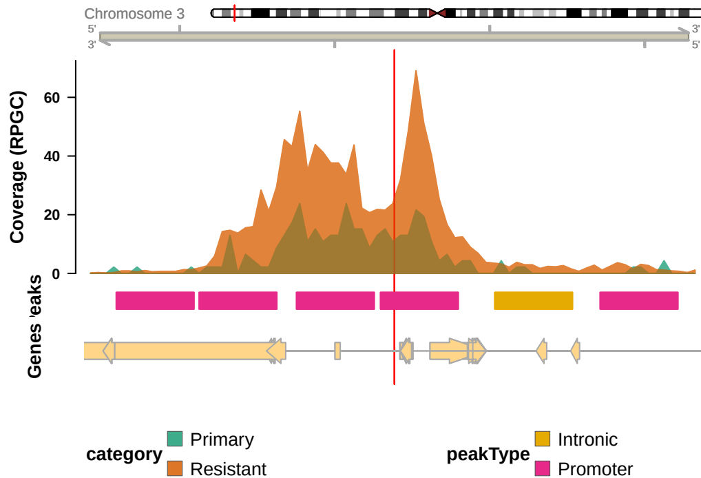
rs2596911 (THUMPD3-AS1),Promoter (&lt;=1kb)
