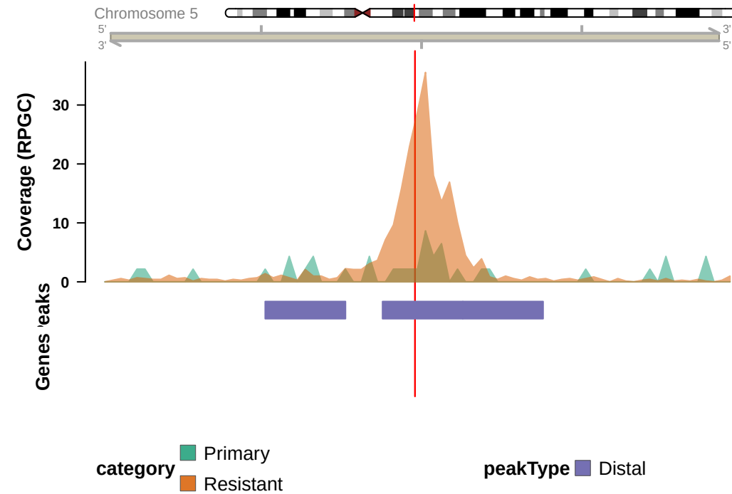
rs1697138 (CD180),Distal Intergenic
