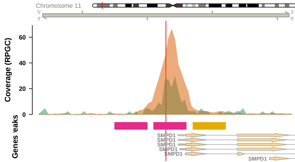
rs538063664 (SMPD1),Promoter (&lt;=1kb)
