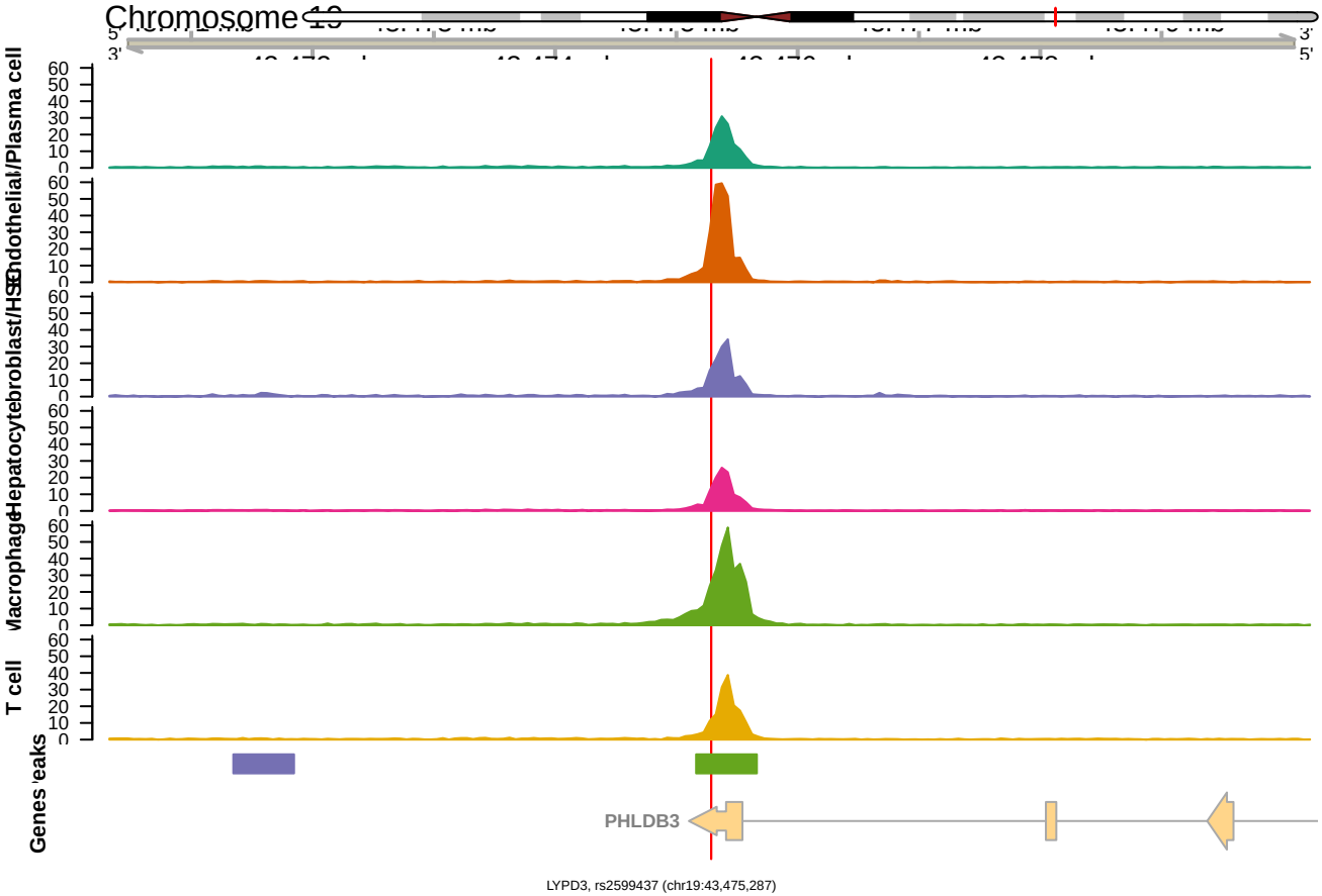
LYPD3, rs2599437 (chr19:43,475,287) +/- 5,000 bp, 50 bp bins (RPGC)
