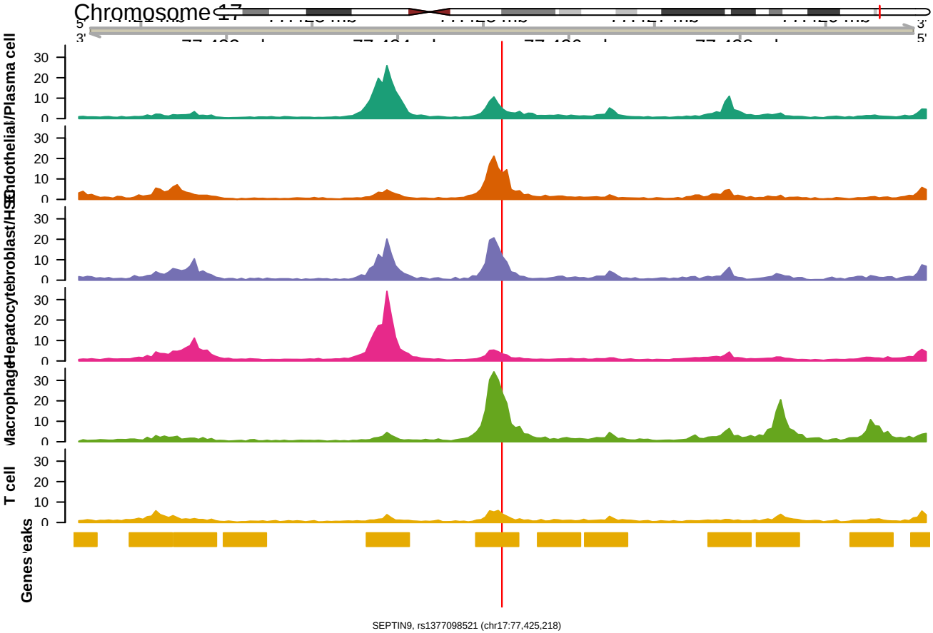
SEPTIN9, rs1377098521 (chr17:77,425,218) +/- 5,000 bp, 50 bp bins (RPGC)
