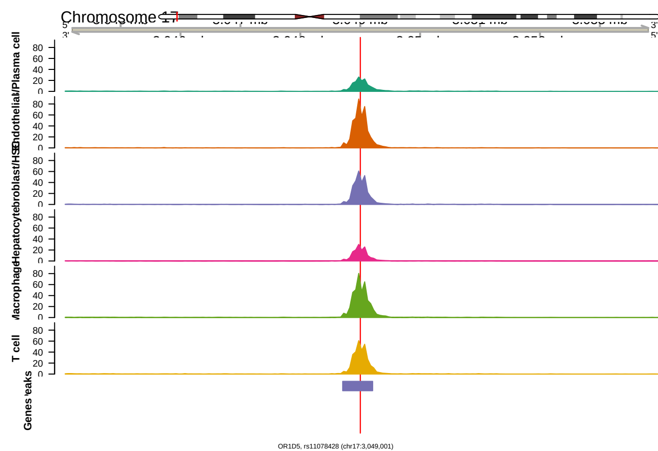
OR1D5, rs11078428 (chr17:3,049,001) +/- 5,000 bp, 50 bp bins (RPGC)
