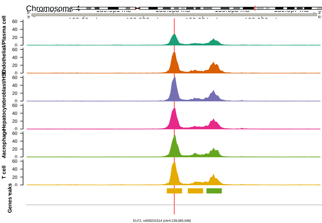
ELF2, rs928231514 (chr4:139,083,048) +/- 5,000 bp, 50 bp bins (RPGC)
