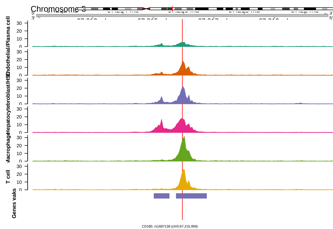
CD180, rs1697138 (chr5:67,215,959) +/- 5,000 bp, 50 bp bins (RPGC)
