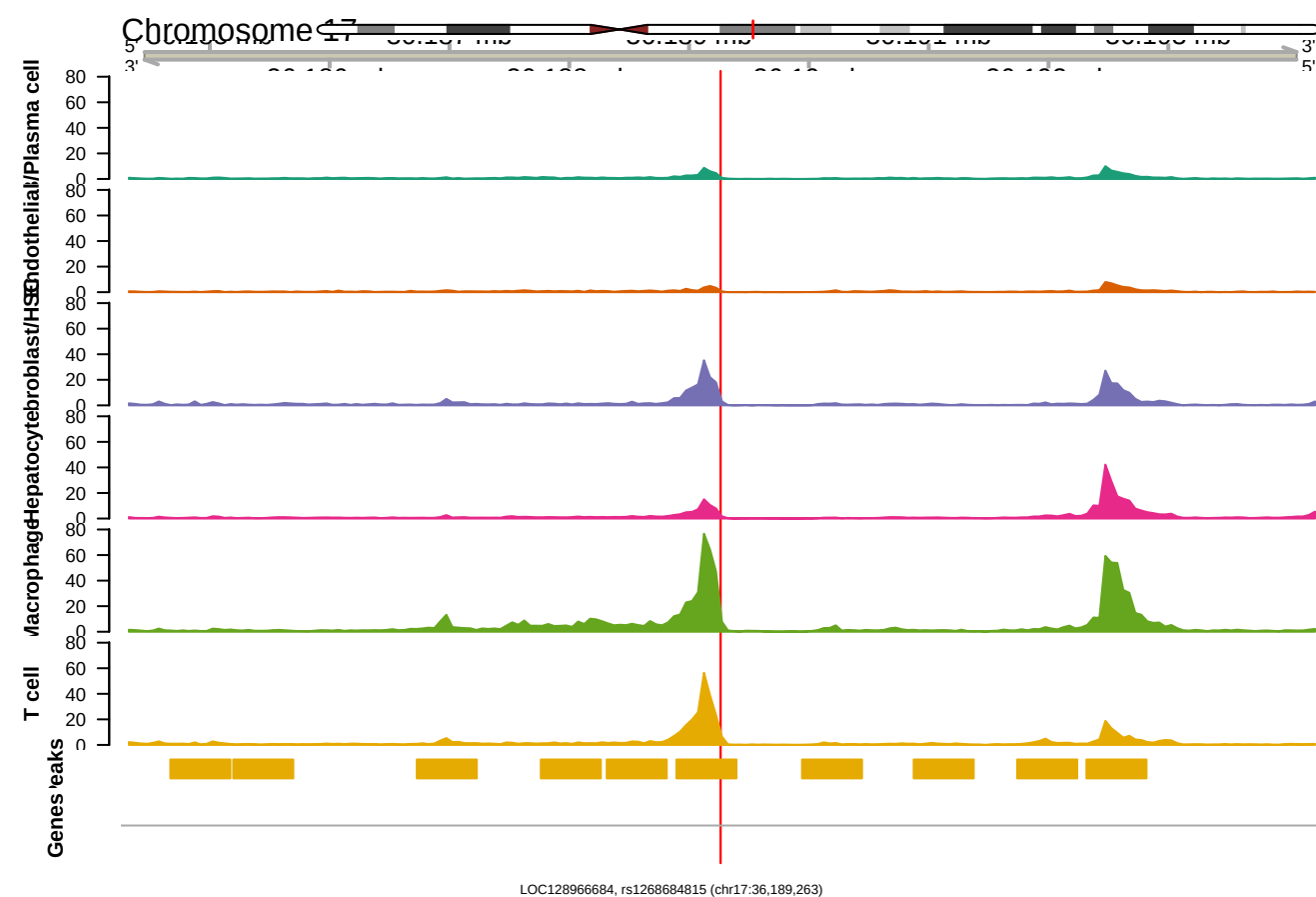
LOC128966684, rs1268684815 (chr17:36,189,263) +/- 5,000 bp, 50 bp bins (RPGC)
