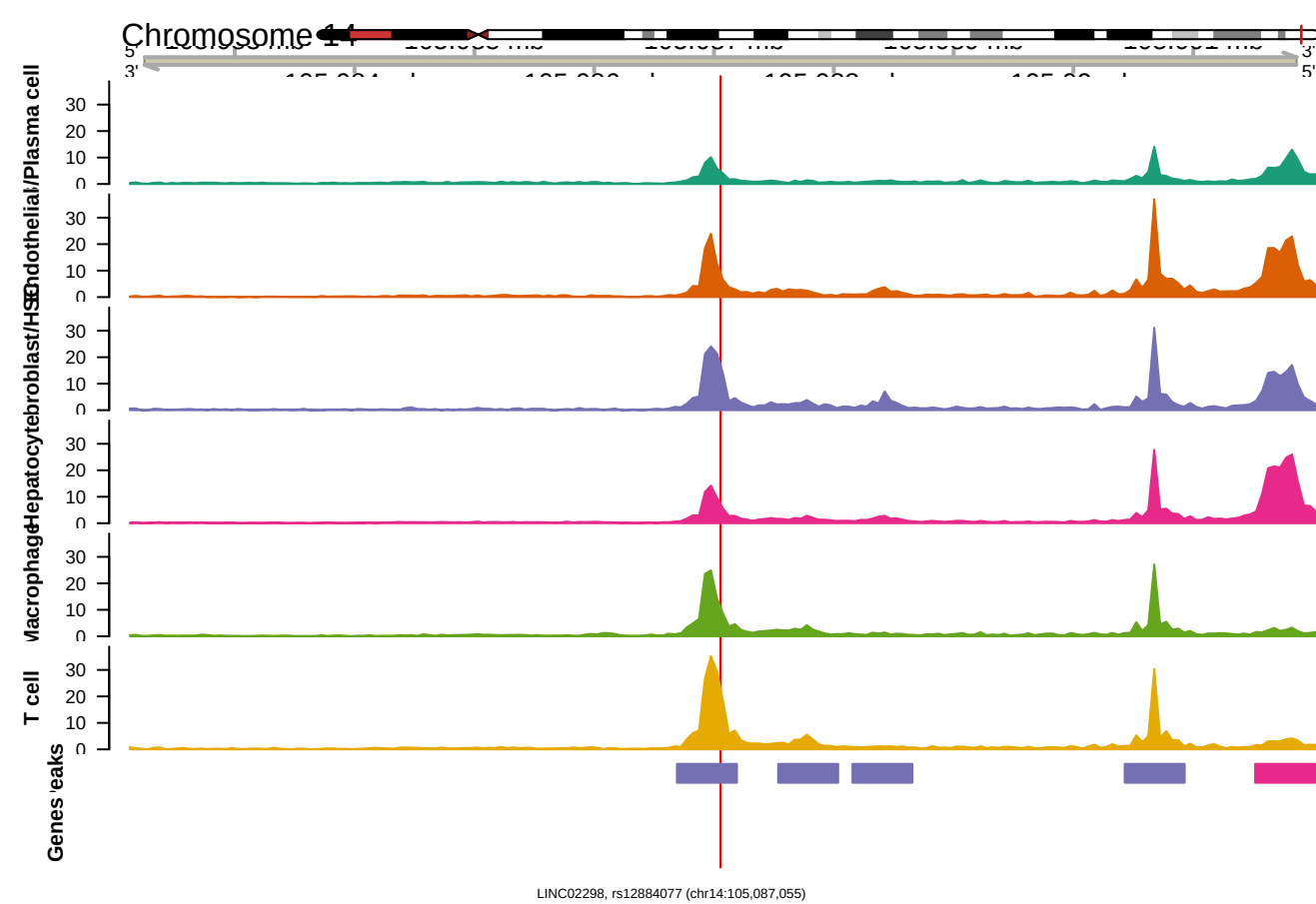
LINC02298, rs12884077 (chr14:105,087,055) +/- 5,000 bp, 50 bp bins (RPGC)
