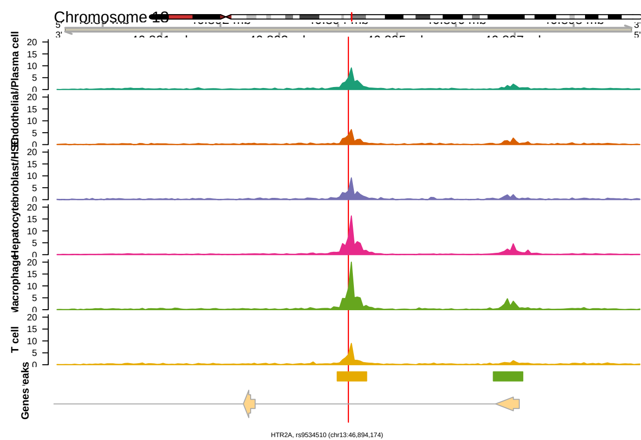
HTR2A, rs9534510 (chr13:46,894,174) +/- 5,000 bp, 50 bp bins (RPGC)
