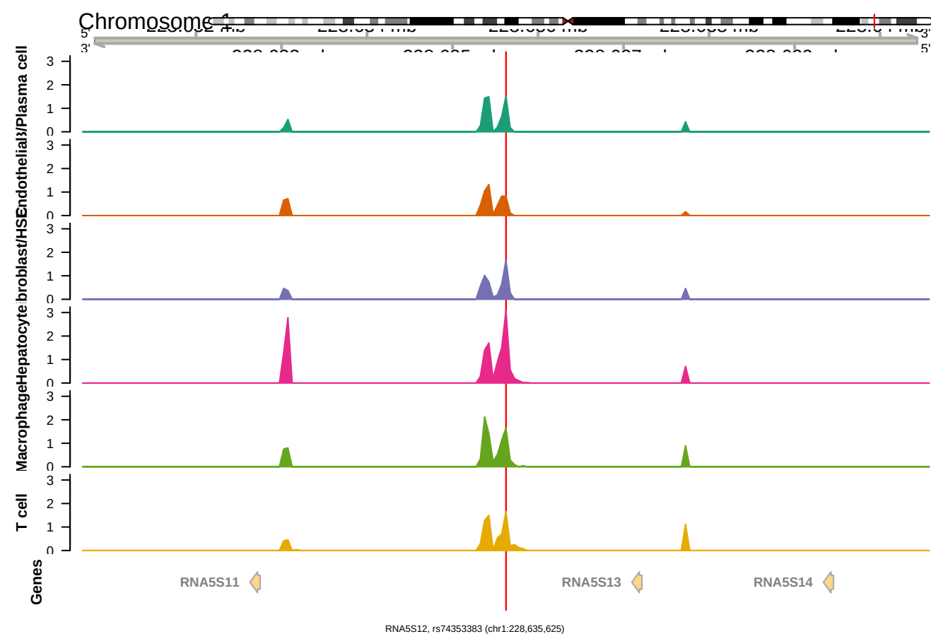
RNA5S12, rs74353383 (chr1:228,635,625) +/- 5,000 bp, 50 bp bins (RPGC)
