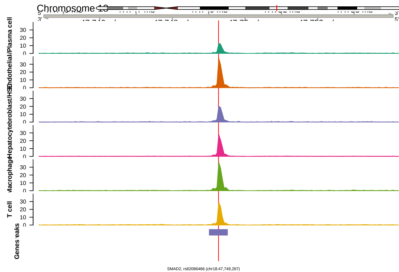
SMAD2, rs62086466 (chr18:47,749,267) +/- 5,000 bp, 50 bp bins (RPGC)
