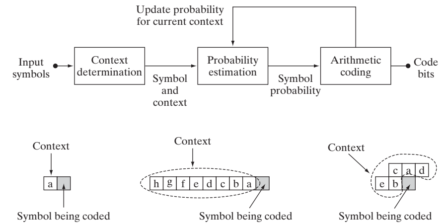
FIGURE 8.13 (a) An adaptive, context-based arithmetic coding approach (often used for binary source symbols). (b)–(d) Three possible context models.
