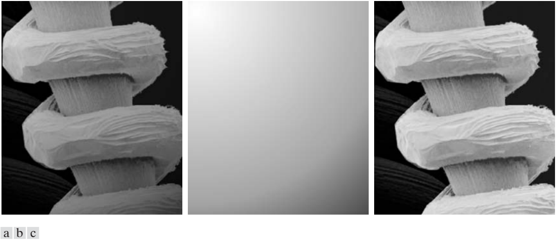
FIGURE 2.29 Shading correction. (a) Shaded SEM image of a tungsten filament and support, magnified approximately 130 times. (b) The shading pattern. (c) Product of (a) by the reciprocal of (b). (Original image courtesy of Michael Shaffer, Department of Geological Sciences, University of Oregon, Eugene.)
