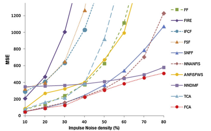
Fig. 8. Performance comparison of selective methods and proposed method as a function of noise ratio for Lena image.
