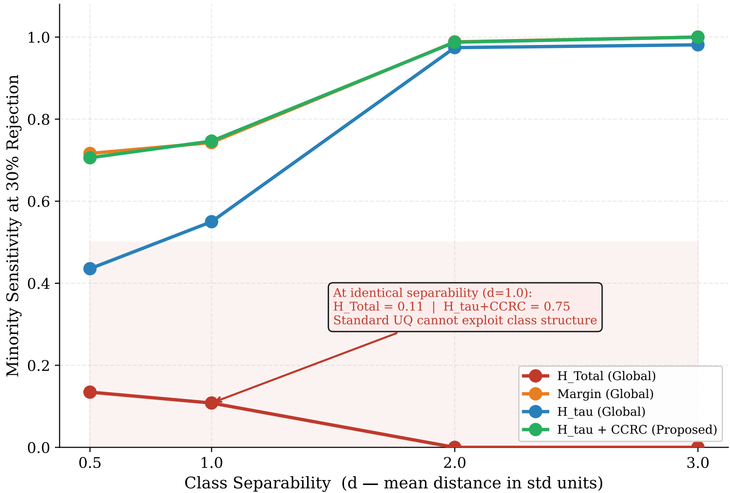
Standard UQ Cannot Exploit Class Separability at Low \tau Even When Progressors Are Biologically Distinct, They Are Rejected ( \tau = 0.10 , N=1000 )
