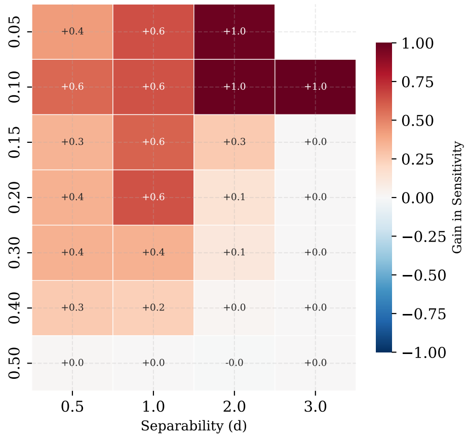
B Recovery: H_{\text{tau}} + CCR
