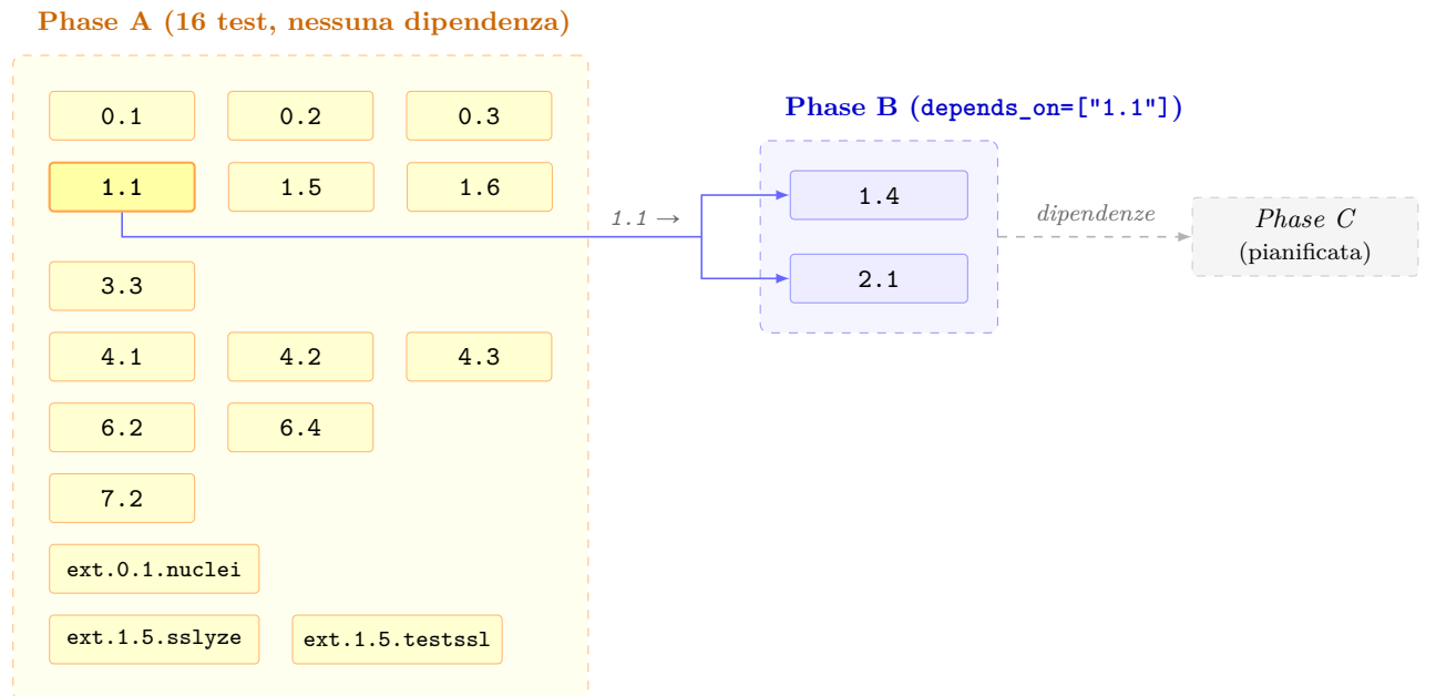
Figura 4.6: Topologia del DAG: Phase A (16 test), Phase B (depends_on=["1.1"]) e Phase C (pianificata).
