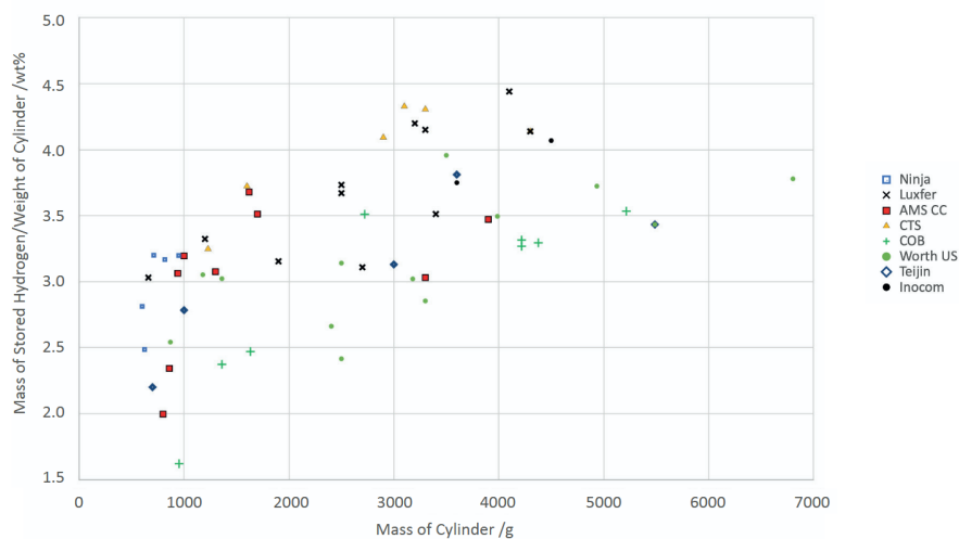
Figure 2.2: Gravimetric Energy Density comparison of hydrogen Cylinders by Intelligent Energy
