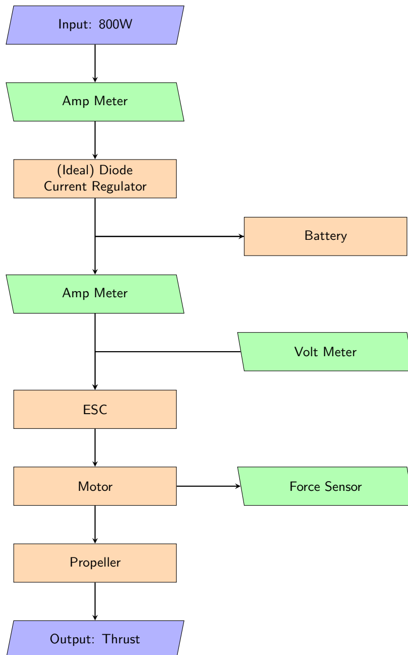
Figure 5.7: Electronics Test Setup
