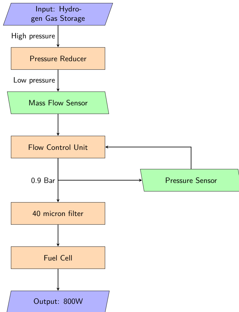
Figure 5.6: Hydrogen Test Setup
