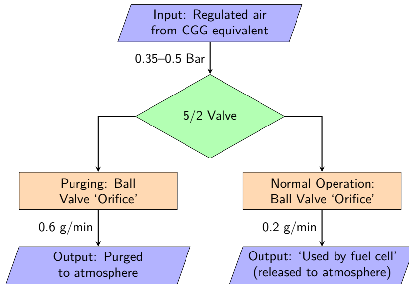
(a) Ball Valve, Single Switch
