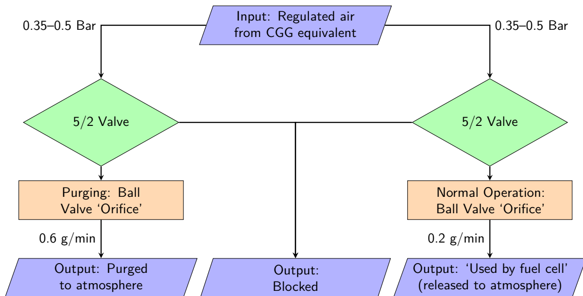
(b) Ball Valve, Dual Switch
