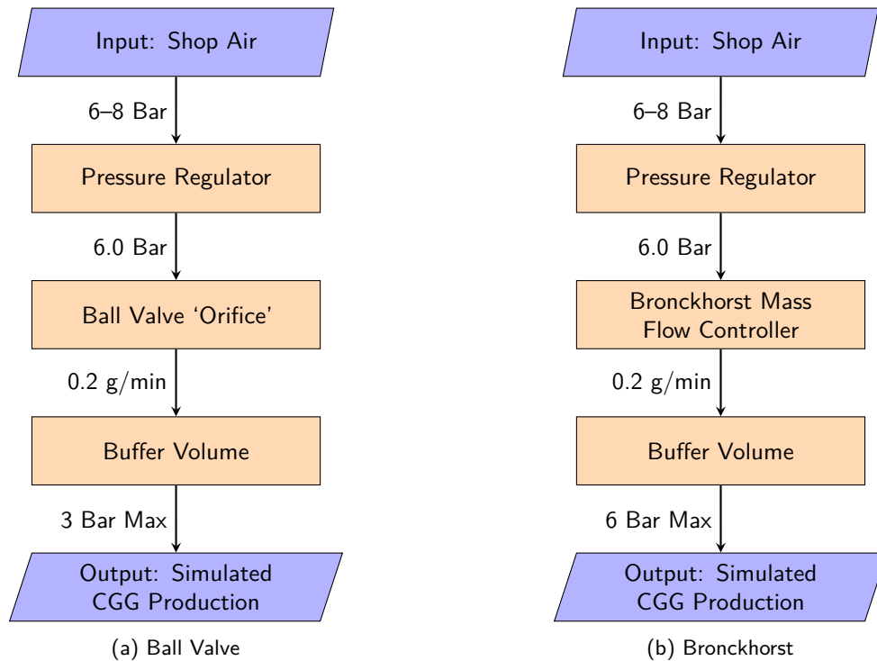
Figure 5.3: CGG Compressed Air Equivalent
