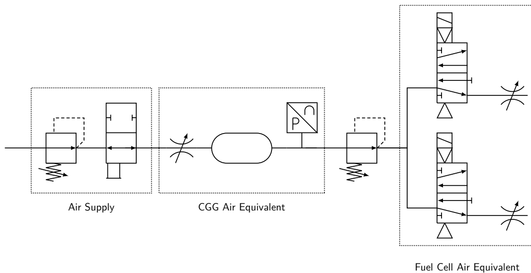
Figure 5.1: Air Test Setup
