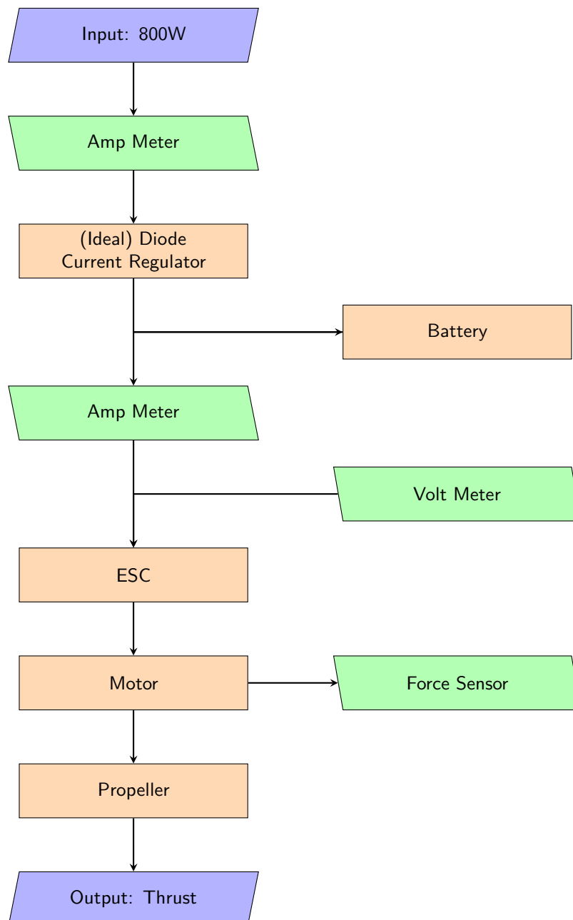
Figure 5.6: Electronics Test Setup
