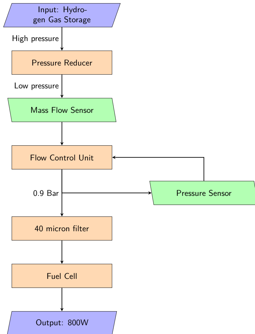
Figure 5.5: Hydrogen Test Setup
