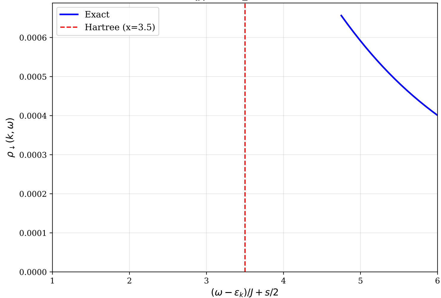
Fig 2: J>0 , k=0 ( s=3.5 , \gamma=1.0 ) W/|J|=10 , \omega_m/W=0.010
