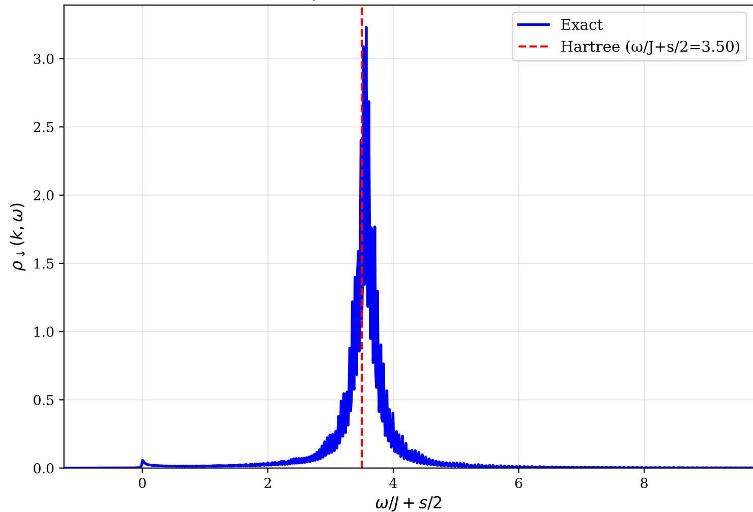
Down-spin spectral weight: J>0 , k=0 ( \gamma=1.0 , s=3.5 , W=10.0 )
