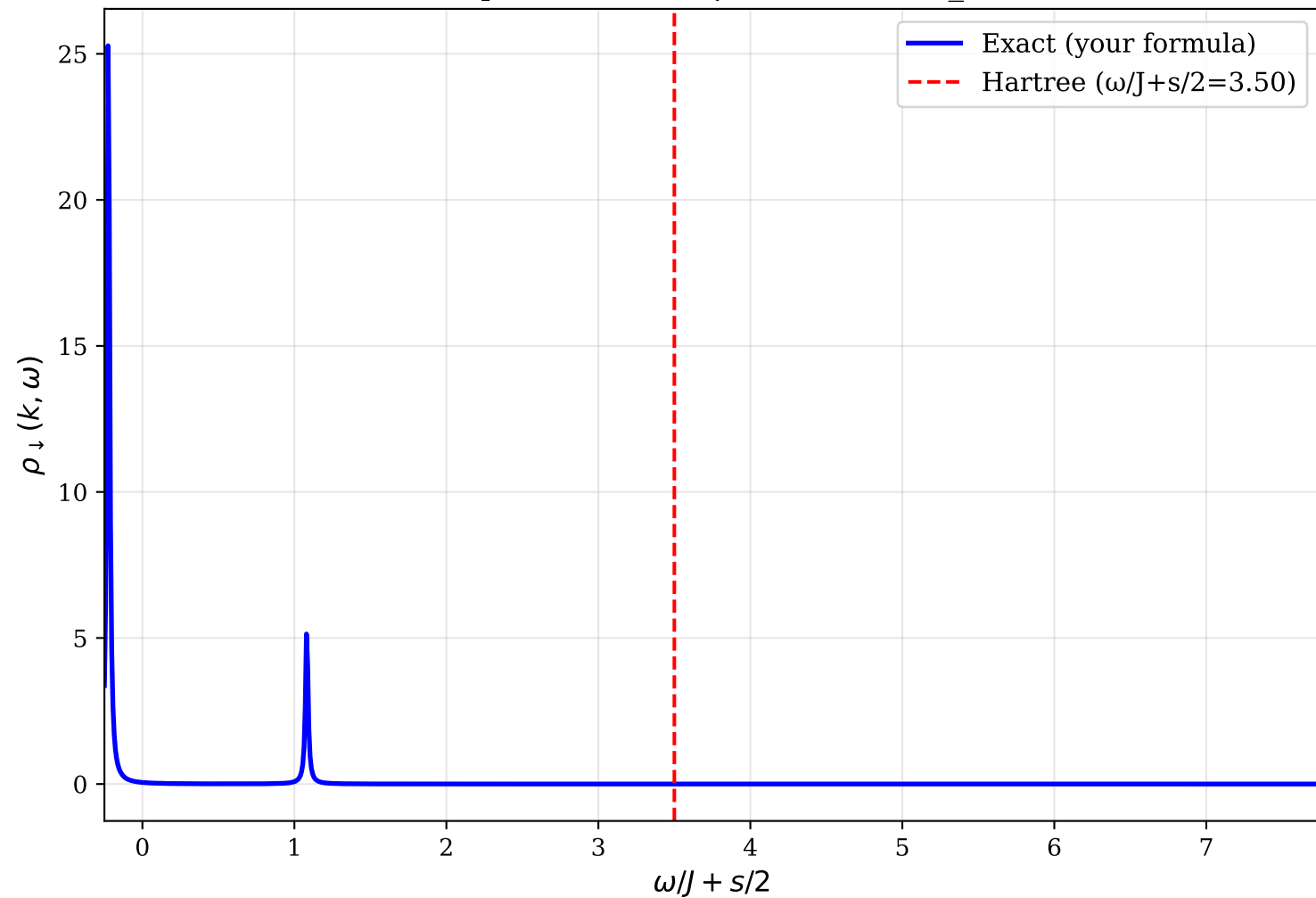
Down-spin spectral weight: J>0 , k=0 Real-space formula ( \gamma=1.0 , s=3.5 , \varepsilon_k=0 )
