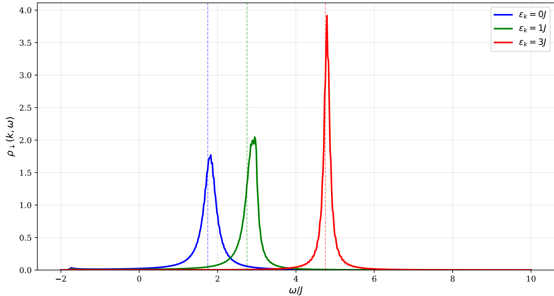
Down-spin spectral weight: J>0 , varying \varepsilon_k ( \gamma=1.0 , s=3.5 , W=10.0 )
