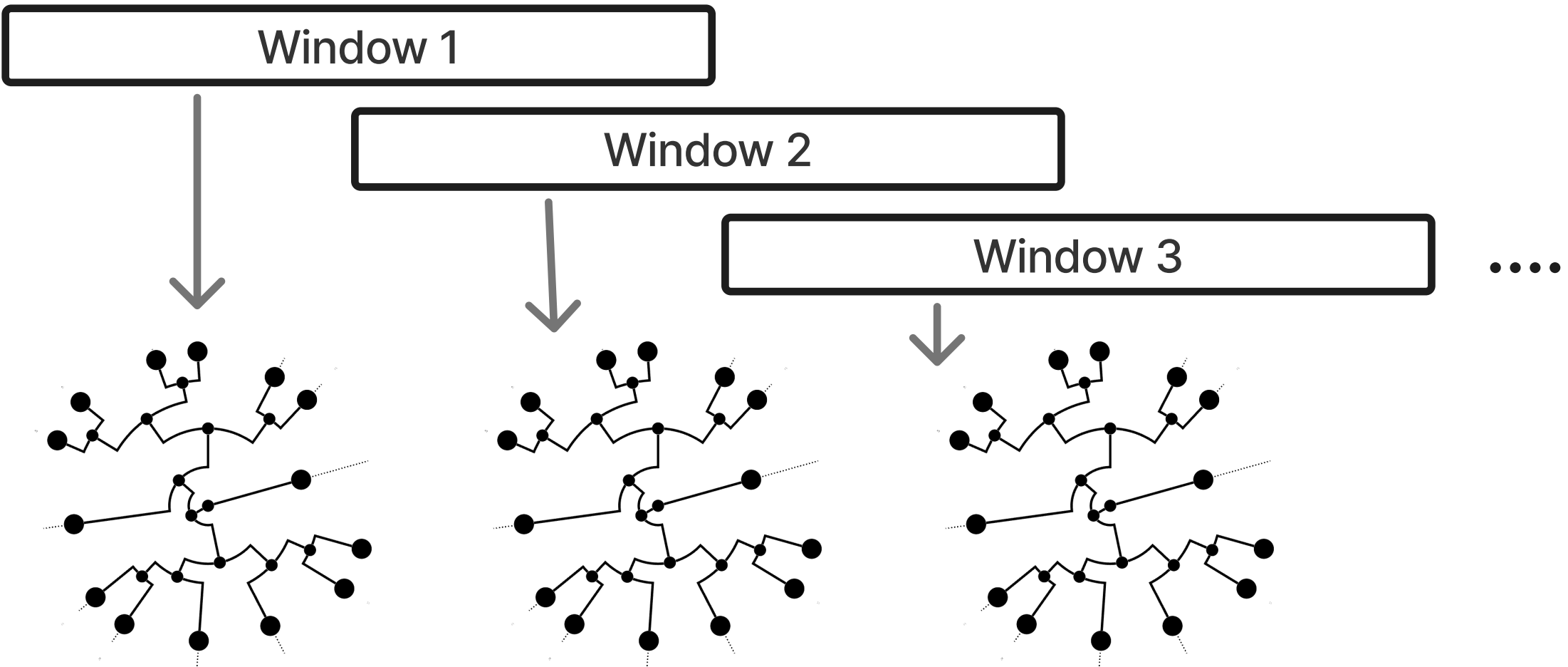
Overlapping Sliding Windows
