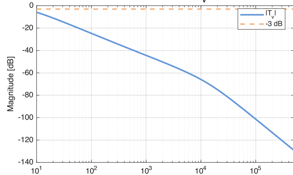
Closed Voltage Loop T_v(s)
