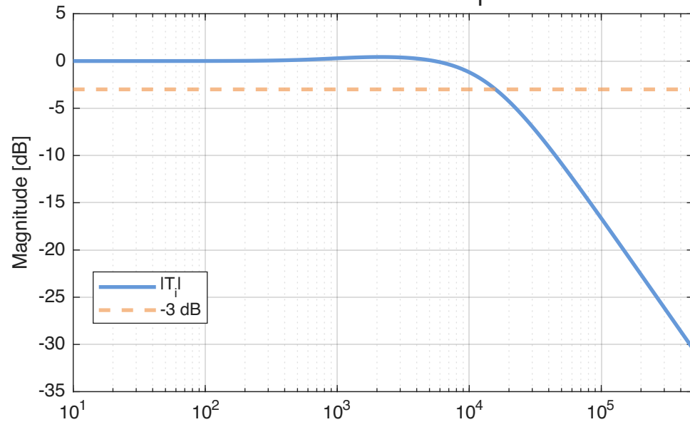
Closed Current Loop T_i(s)
