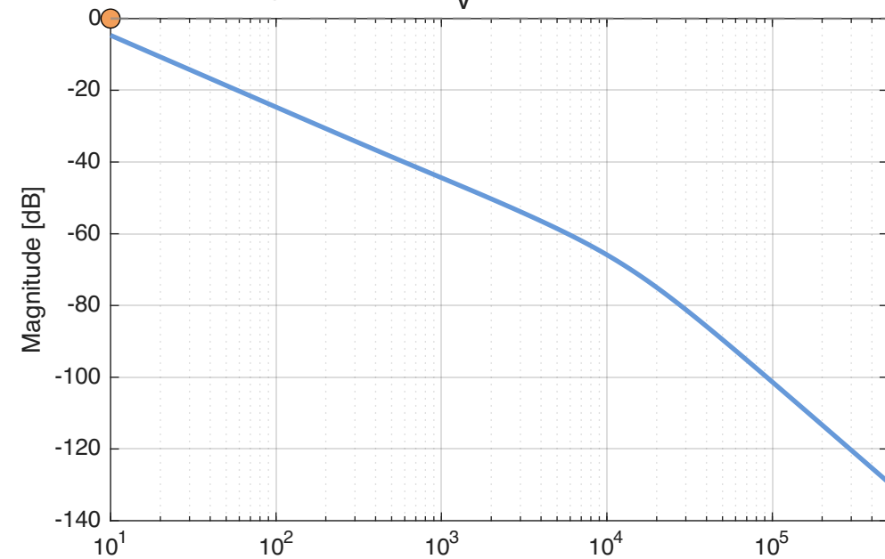
Voltage Open Loop L_v(s) | GM = \infty , PM = 87.6°
