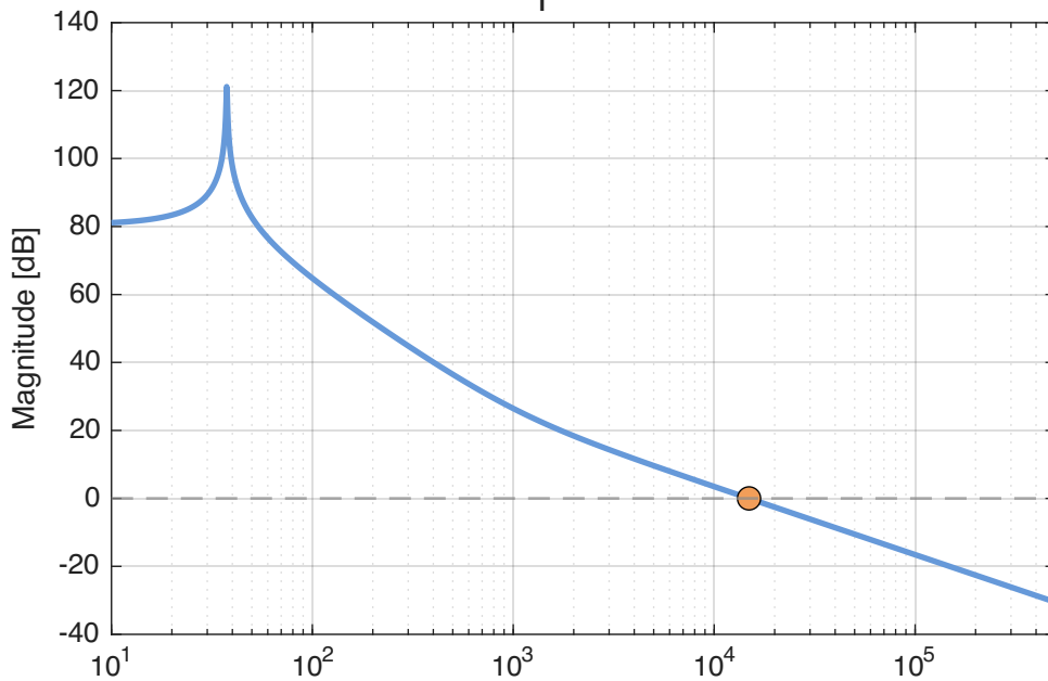
Current Open Loop L_i(s) | GM = \infty , PM = 86.2°
