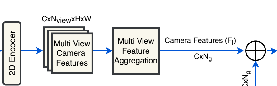
Surround-View Images
