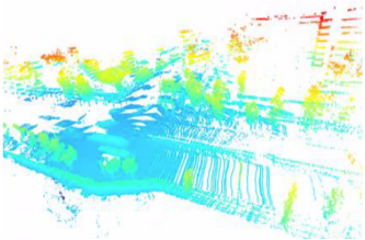
LiDAR Points
