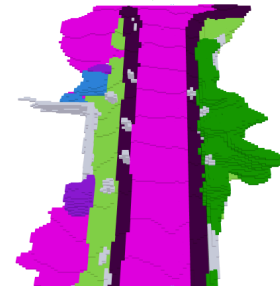
Occupancy Prediction
