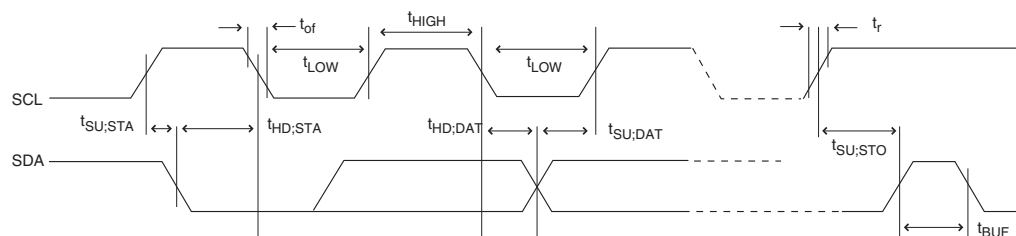
Figure 145. Two-wire Serial Bus Timing
