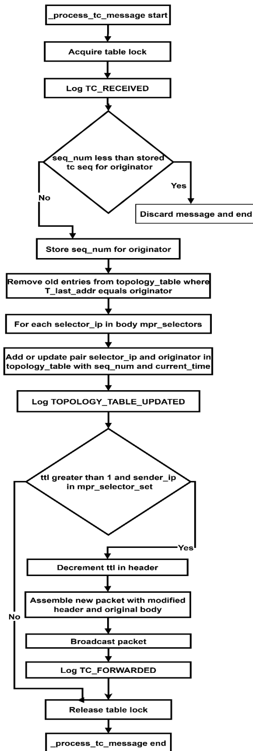
Figure B.13 Detailed Implementation Flow of TC Message Processing
