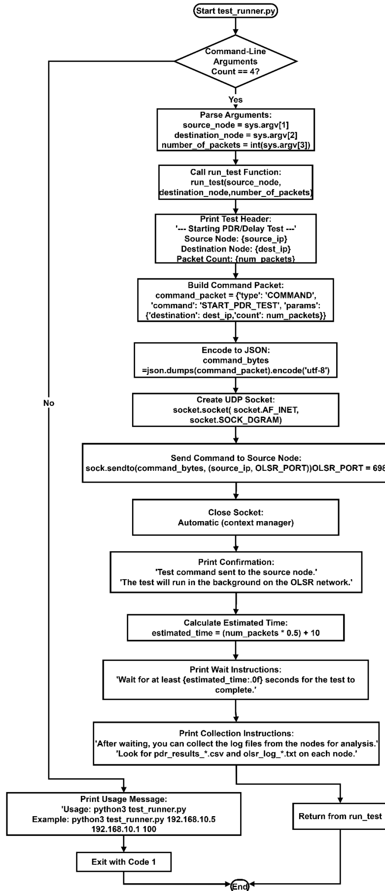
Figure B.22: Detailed Implementation Flow of the External Traffic Generator Script
