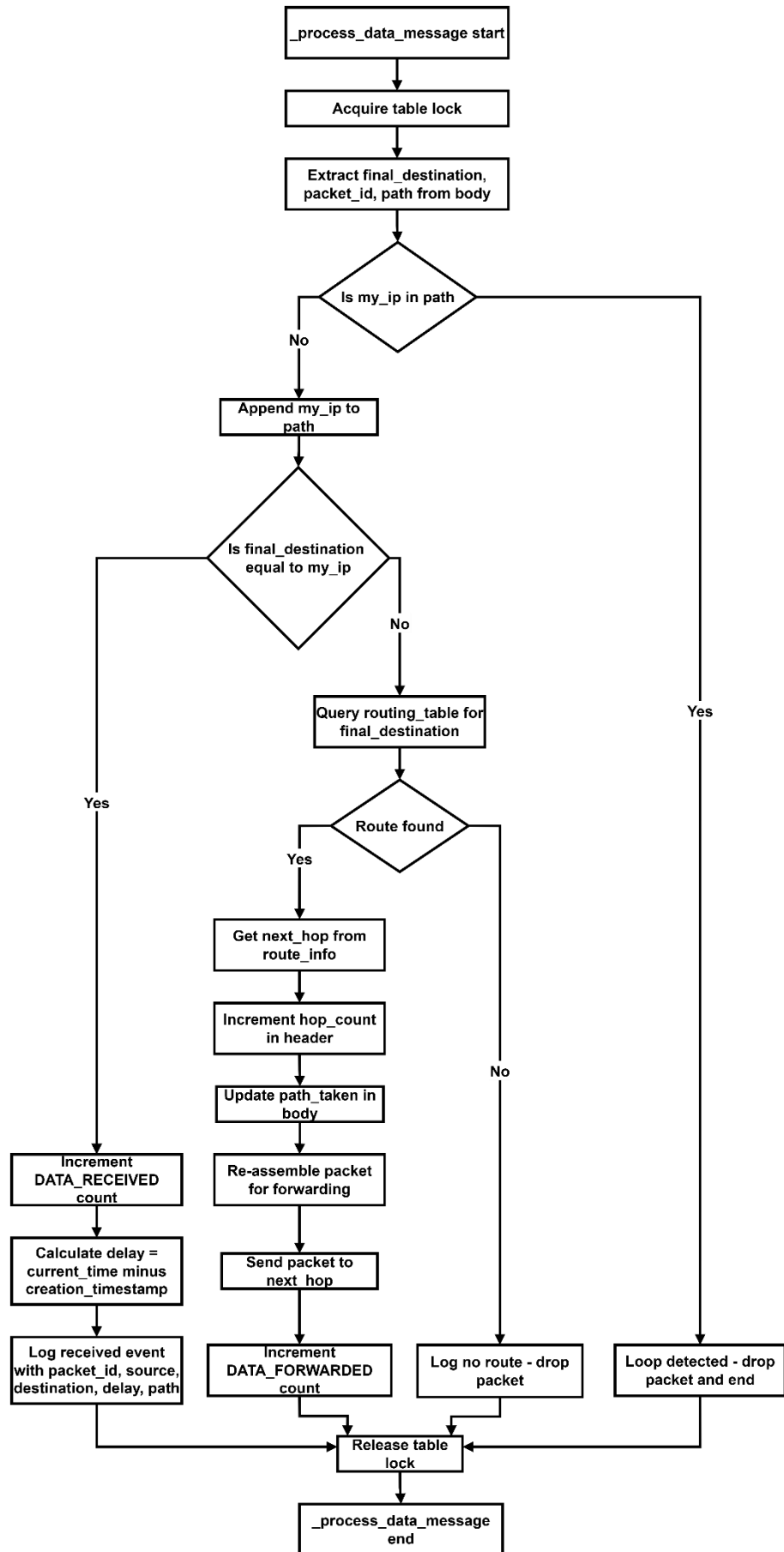
Figure B.16: Detailed Implementation Flow of DATA Message Processing
