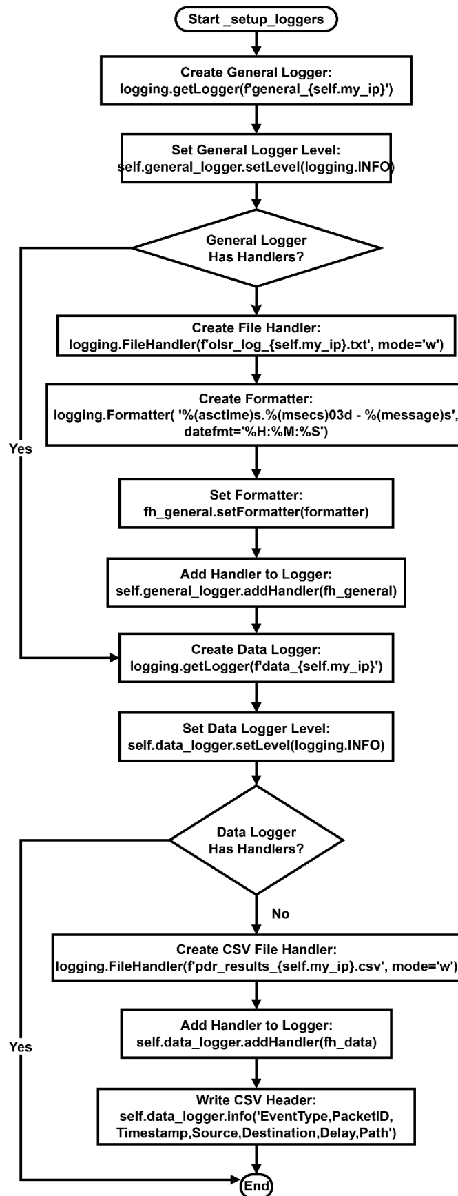
Figure B.21 Detailed Implementation Flow of Logging Infrastructure Setup
