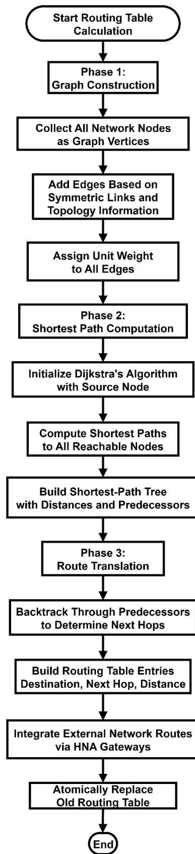
Figure B.18: Conceptual Design of Routing Table Calculation
