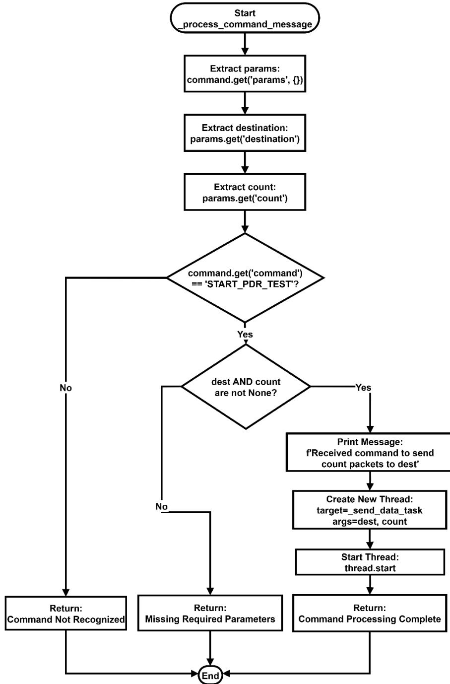
Figure B.17: Detailed Implementation Flow of Command Message Processing
