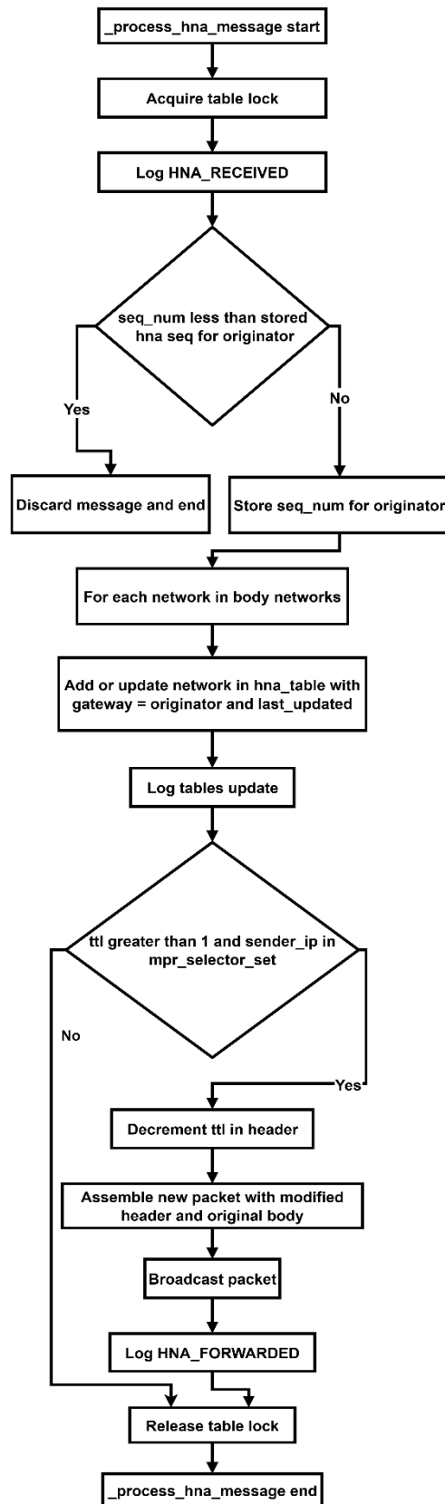
Figure B.14 :Detailed Implementation Flow of HNA Message Processing
