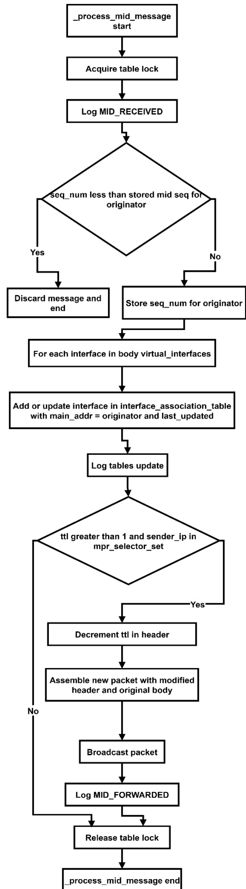
FigureB.15:Detailed Implementation Flow of MID Message Processing
