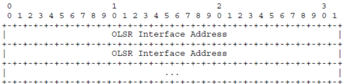
Figure A. 4:MID Message body fields
