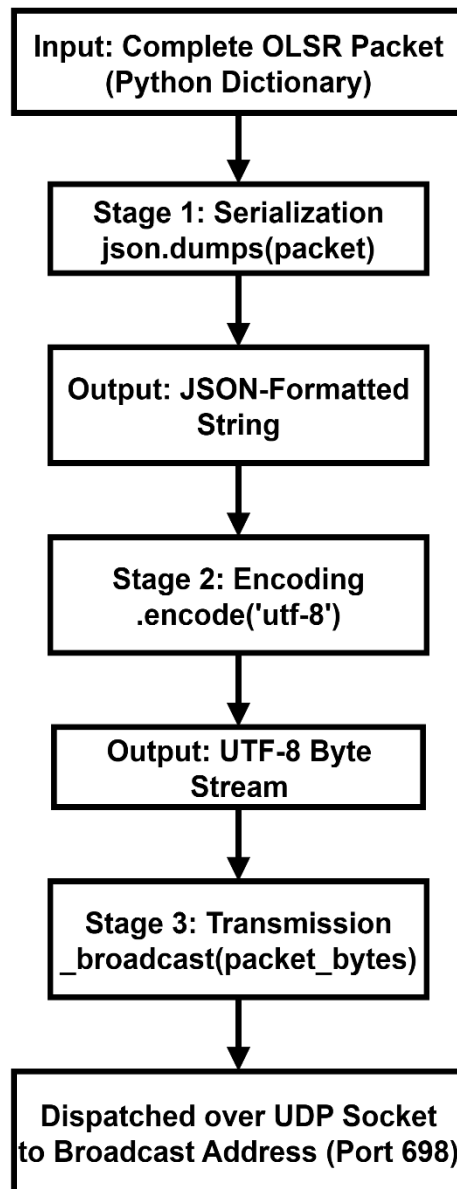
Figure A.3 The packet serialization and transmission process
