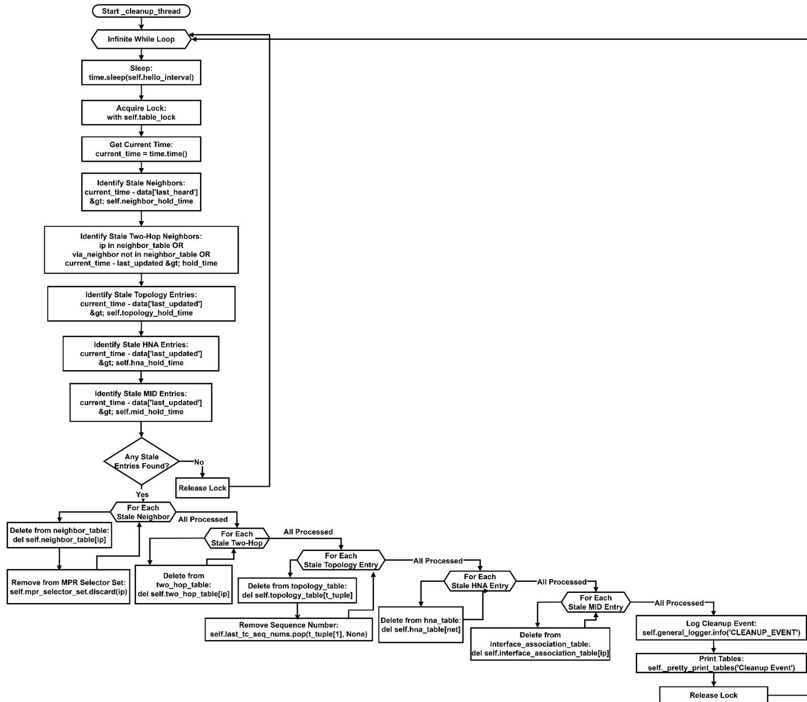
Figure A.17: Detailed Implementation Flow of the Cleanup Thread
