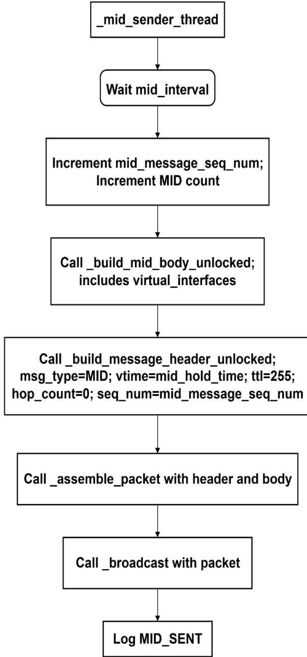
Figure A.6: MID Sender Thread
