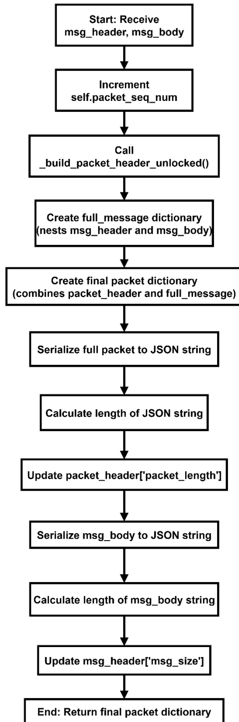
Figure A.2 Flowchart of the _assemble_packet() method
