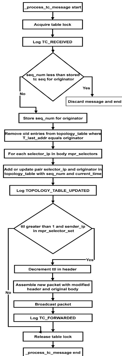
Figure A. 11 Detailed Implementation Flow of TC Message
