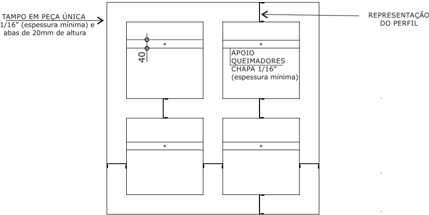
CHAPA SUPERIOR
