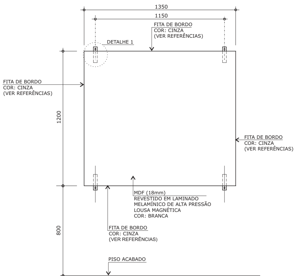
VISTA FRONTAL
