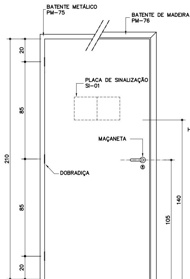
VISTA 1 – EXTERNA
