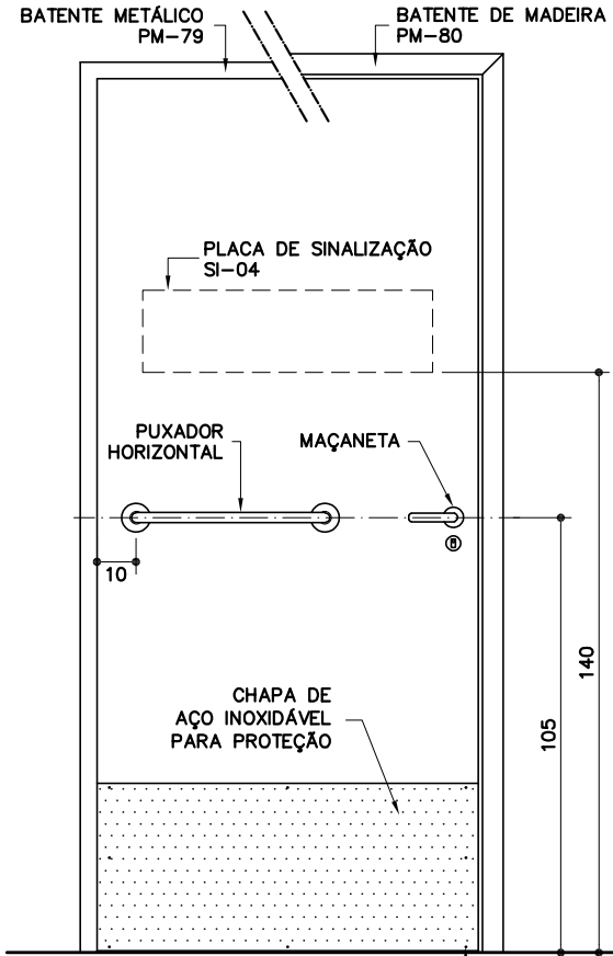
VISTA 3 – EXTERNA
