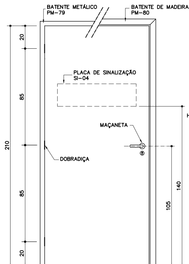
VISTA 1 – EXTERNA
