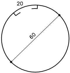
N1 11Ø6.3 c/20 C=225
