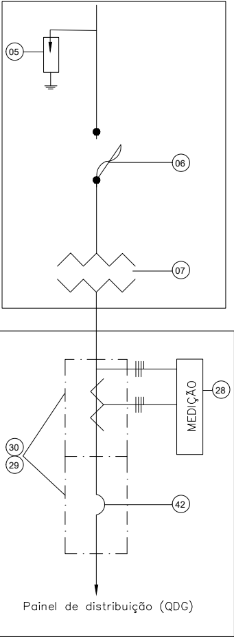
DIAGRAMA UNIFILAR
