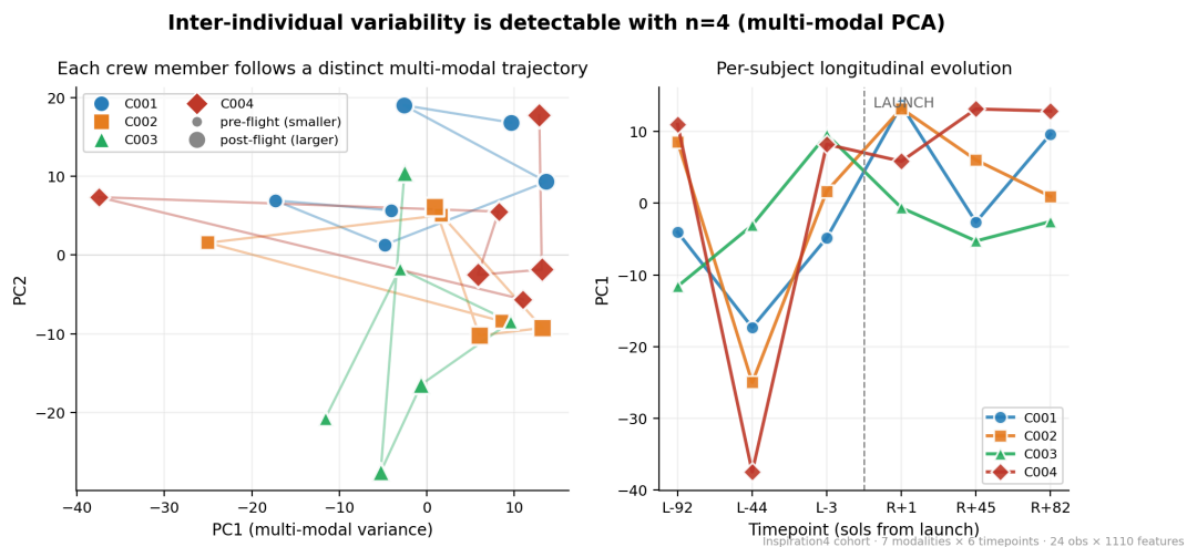
Figure 2: Inter-subject latent-state trajectories from the multi-modal factor model ( K=2 latent dimensions, seven modalities, 1110 features). Each colour traces one Inspiration4 crew member from L-92 (pre-launch) through R+82 (post-flight). The displacement of all four trajectories along latent dimension 1 between L-3 and R+1 is consistent with a flight-induced shift; the orthogonal between-subject spread on latent dimension 2 captures inter-individual variability resolvable even at n=4 .
