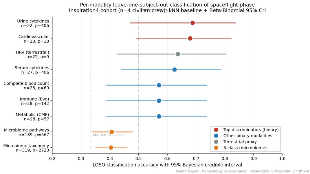
Figure 1: Headline LOSO accuracy across the nine modalities. Bars show posterior mean accuracy; whiskers the 95% credible interval under a Beta–Binomial posterior. Modalities below the 0.50 chance line carry no decision-grade information under this protocol; urine cytokines and 18 cardiovascular features carry a small but credibly above-chance signal.
