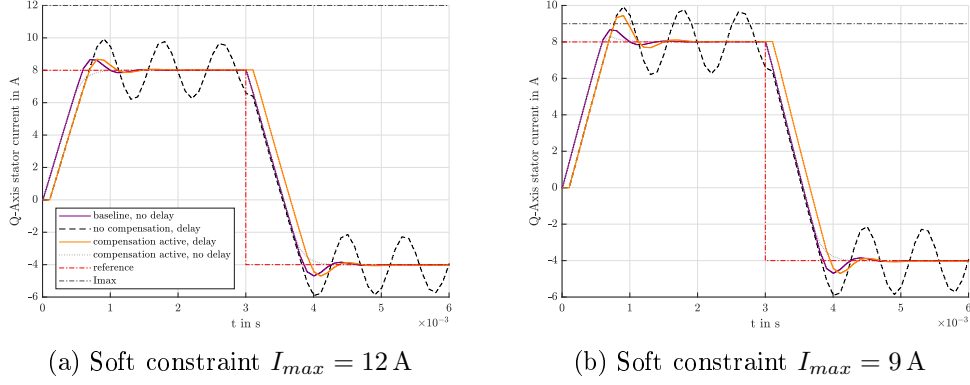
Figure 2.13: Simulated step responses for deadtime scenarios with the Basic MPC
