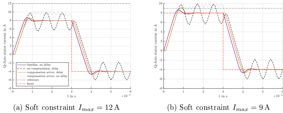
Figure 2.15: Simulated step responses for deadtime scenarios with the Hybrid MPC
