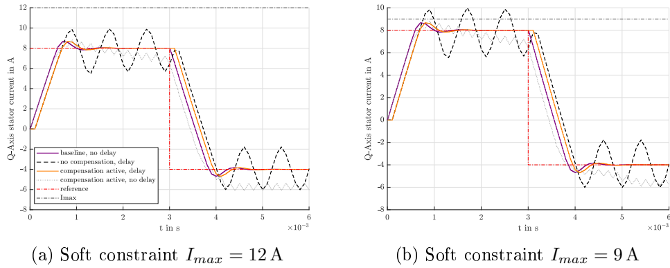
Figure 2.14: Simulated step responses for deadtime scenarios with the Embedded Integrator MPC due to Wang
