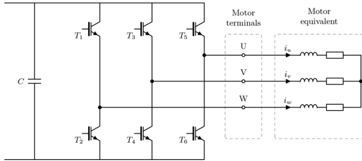
Figure 2.17: Two-level inverter driving the PMSM and induction machine. Image source: [15]
