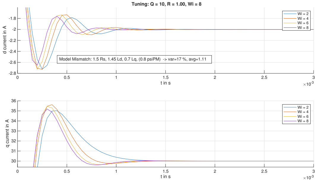
Figure 2.16: Comparison of the step responses for multiple values of W_I considering model fault
