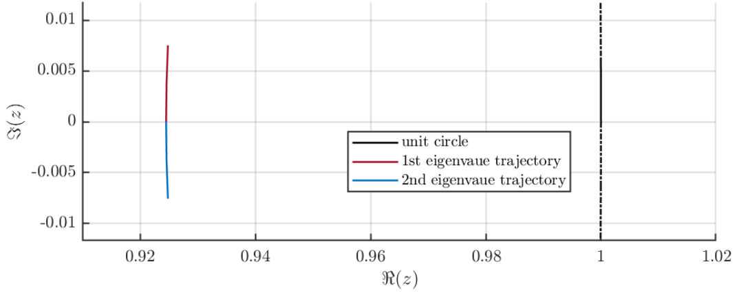
Figure 2.8: Spectrum of \mathbf{A}_{C,b}(\omega) for \omega \in \mathcal{W} of the unconstrained Basic MPC.
