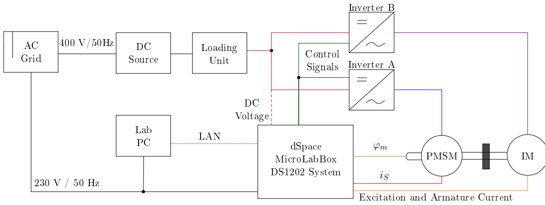
Figure 2.18: Schematic of the end-to-end test bed for the MPC tests at TUG
