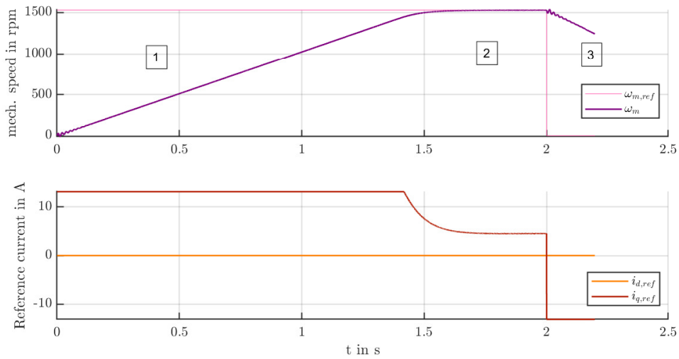
Figure 2.17: Simulated speed ramp: reference quantities
