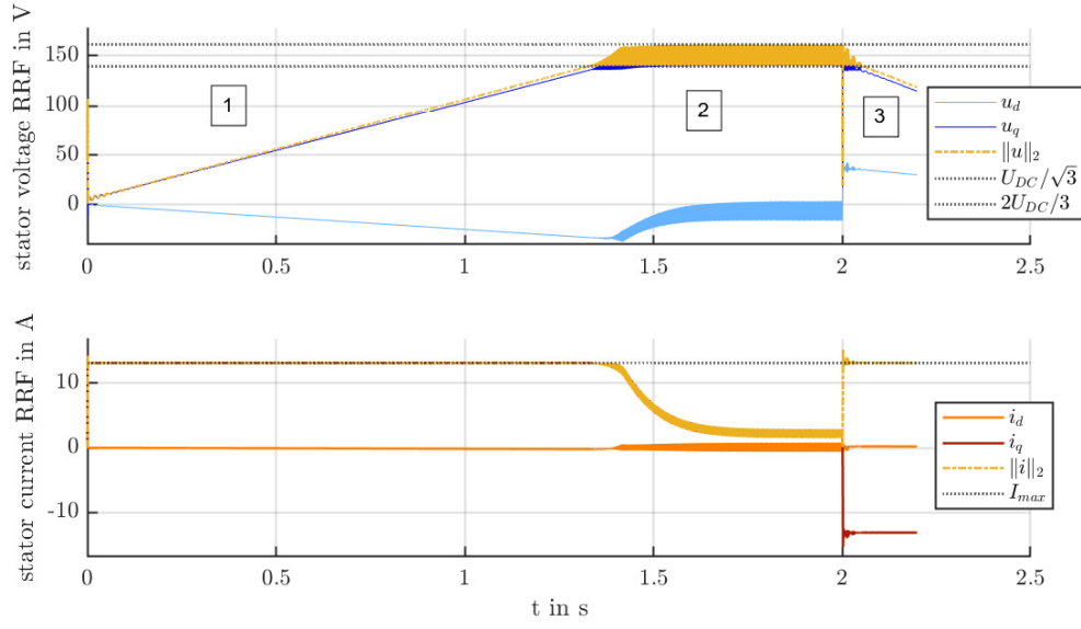
Figure 2.18: Simulated speed ramp: control quantities
