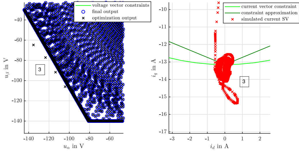
Figure 2.20: Simulated speed ramp: voltage and current constraints, detail during deceleration phase
