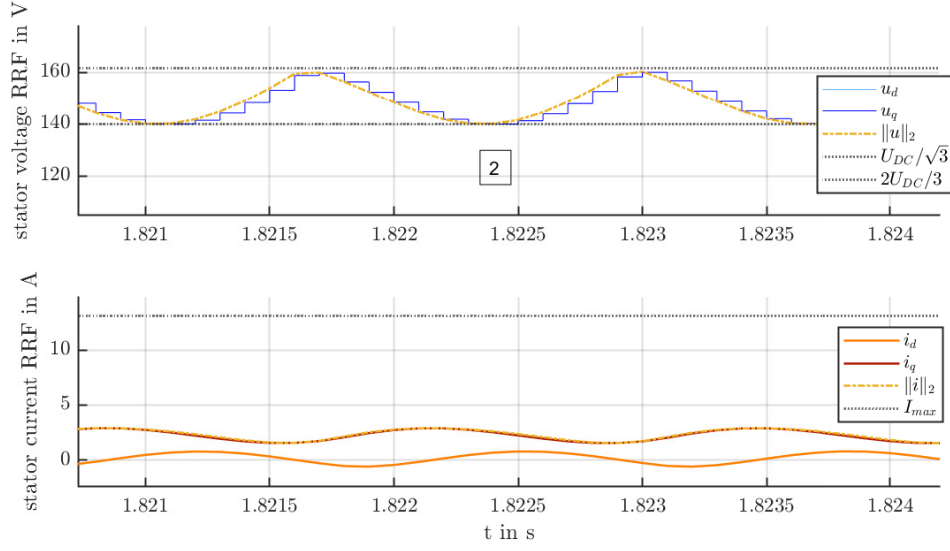
Figure 2.22: Simulated speed ramp: Phase 2 - Over-modulation due to active voltage constraints
