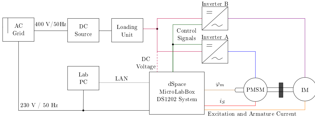
Figure 2.25: Schematic of the end-to-end test bed for the MPC tests at TUG
