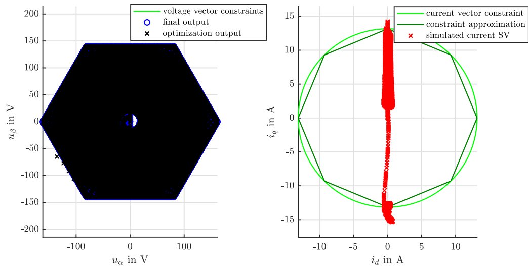
Figure 2.19: Simulated speed ramp: voltage and current constraints
