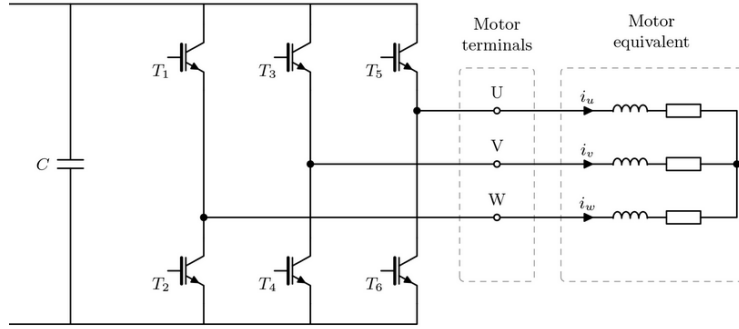
Figure 2.24: Two-level inverter driving the PMSM and induction machine. Image source: [15]
