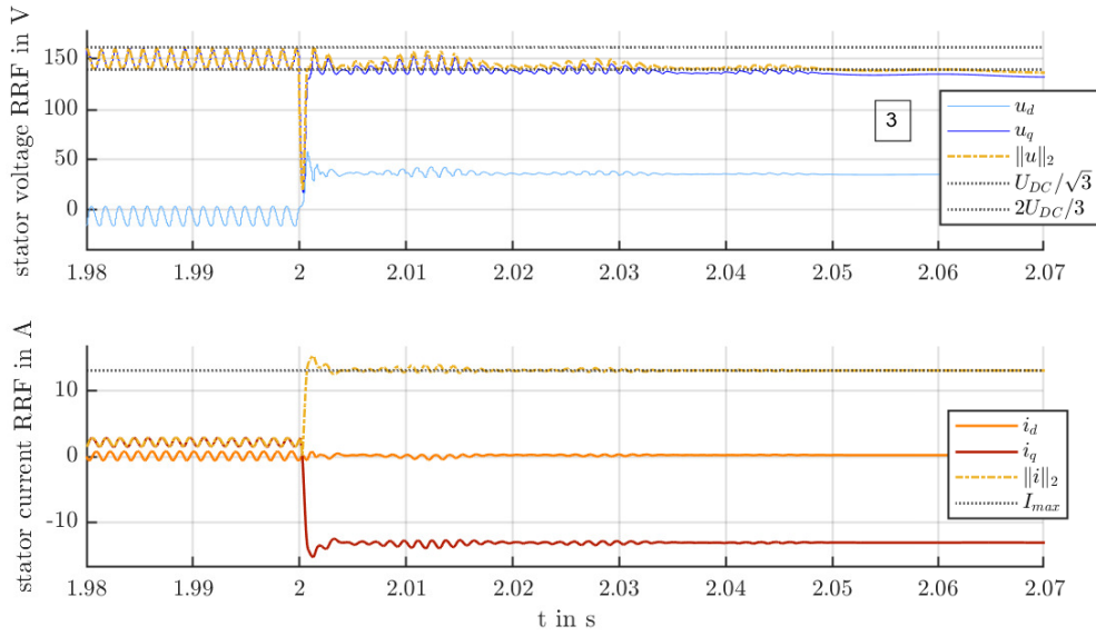
Figure 2.23: Simulated speed ramp: Phase 3 - Deceleration
