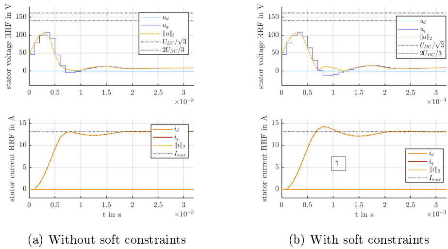
Figure 2.21: Simulated speed ramp: Phase 1 - Acceleration
