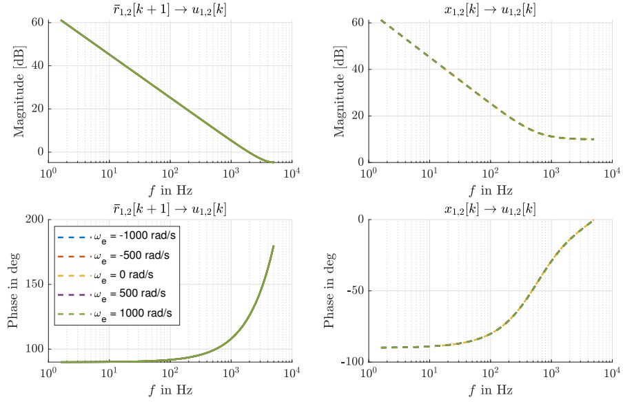
Figure 3.5: Frequency response for the unconstrained Hybrid MPC.
