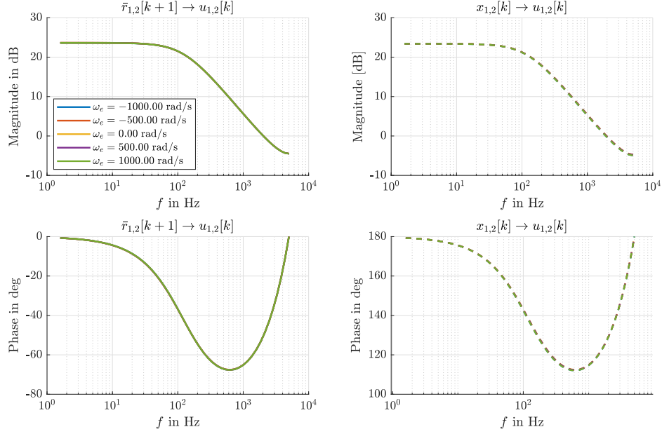
Figure 3.6: Frequency response for the unconstrained Basic MPC.
