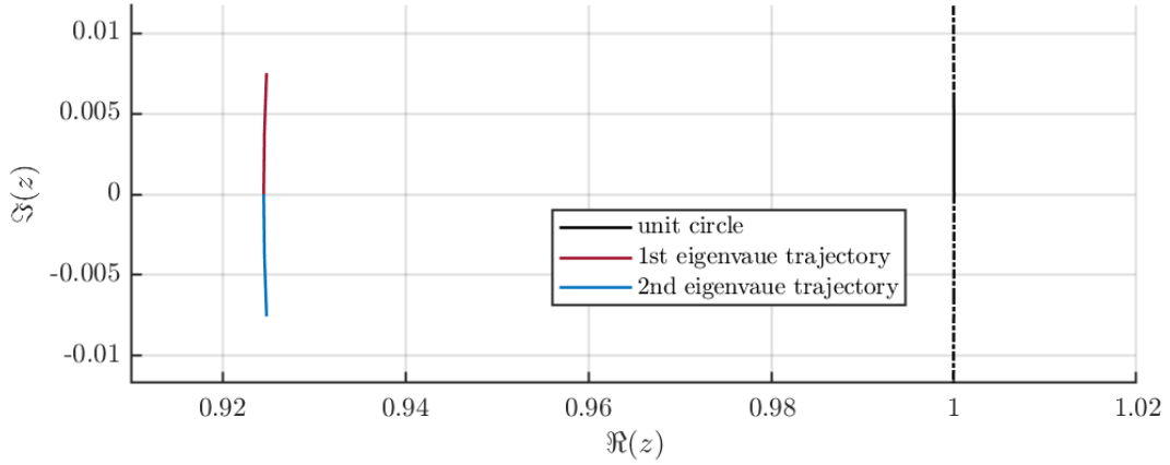
Figure 3.5: Spectrum of \mathbf{A}_{C,b}(\omega) for \omega \in \mathcal{W} of the unconstrained Basic MPC.
