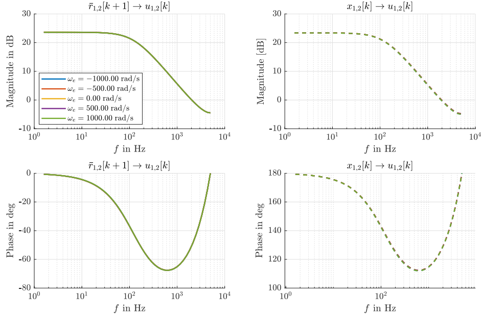
Figure 3.6: Frequency response for the unconstrained Basic MPC.
