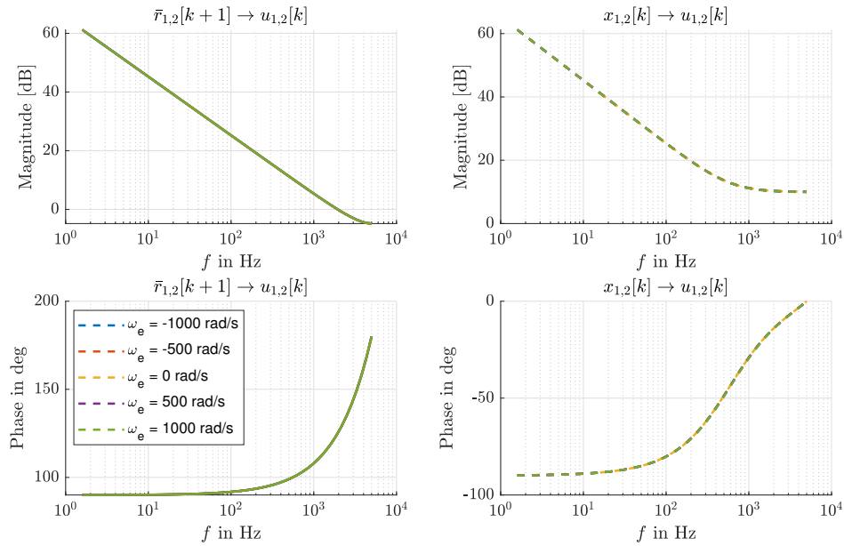
Figure 3.8: Frequency response for the unconstrained Hybrid MPC.
