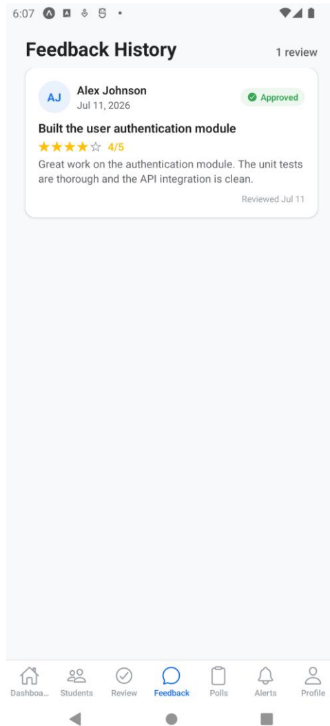
Figure 26. Feedback history
