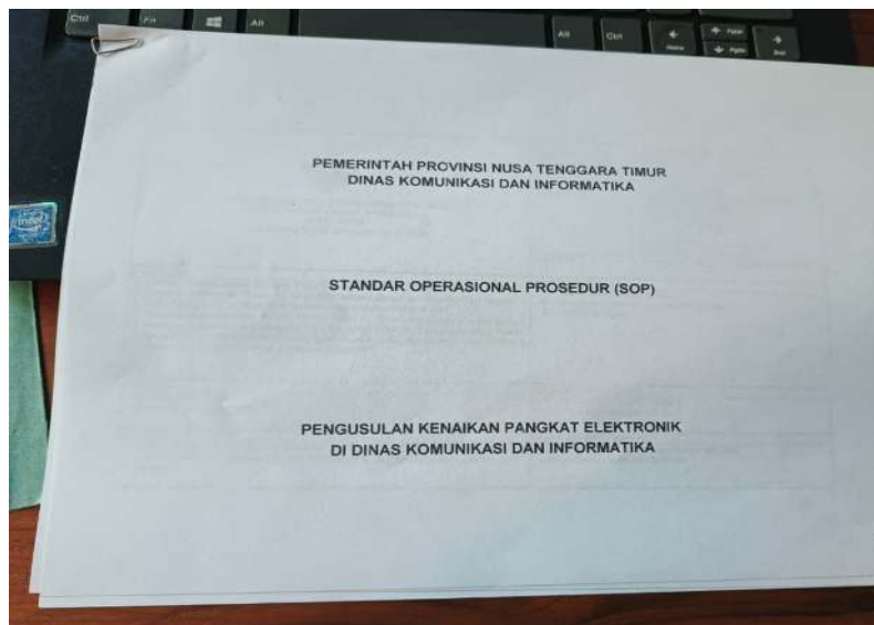
Gambar 13. Draft SOP
