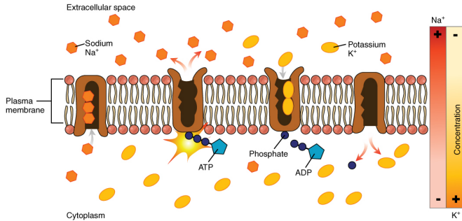
Sodium-potassium ATPas, from OpenStax Anatomy and Physiology via Wikimedia
