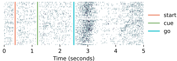
Neuron 17 go-cue aligned spikes
