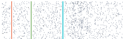
Neuron 17 go-cue aligned spikes
